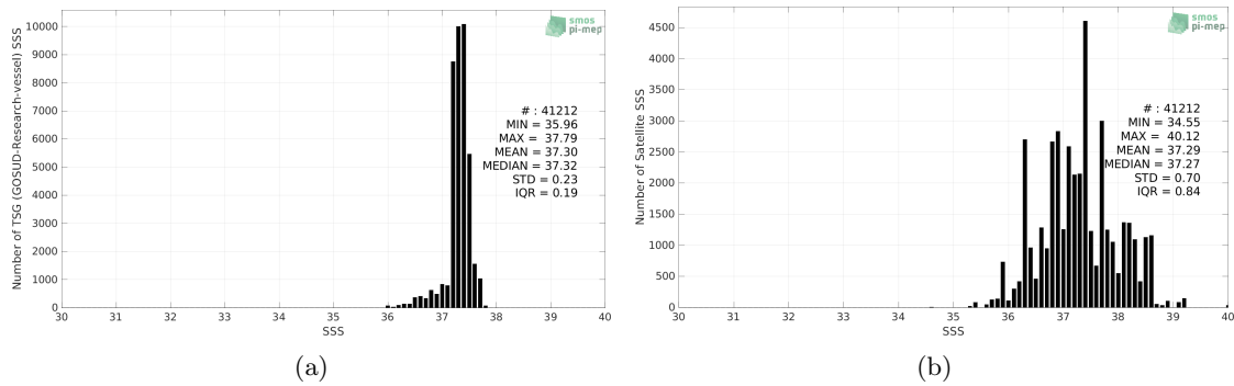
Figure 2: Histograms of SSS from TSG (GOSUD-Research-vessel) (a) and SMOS SSS L2Q v331 - 0.25 Deg (CATDS-CPDC) (b) considering all match-up pairs per bins of 0.1 over the SPURS 1 Pi-MEP region and for the full satellite product period.
