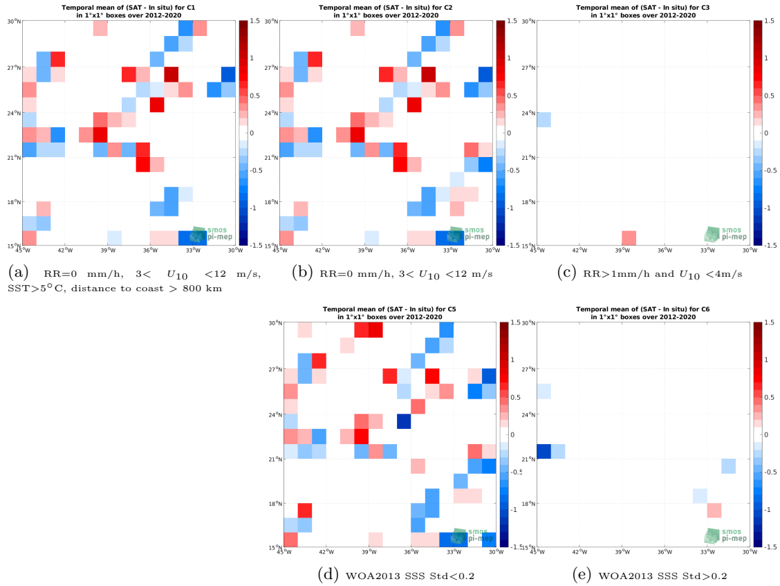
Figure 12: Temporal mean gridded over spatial boxes of size 1^{\circ} \times 1^{\circ} of \Delta\text{SSS} (SMOS SSS L2Q v331 - 0.25 Deg (CATDS-CPDC) - TSG (GOSUD-Research-vessel)) for 5 different subdatasets corresponding to: RR=0 mm/h, 3 < U_{10} < 12 m/s, SST > 5^{\circ}\text{C} , distance to coast > 800 km (a), RR=0 mm/h, 3 < U_{10} < 12 m/s (b), RR > 1\text{mm/h} and U_{10} < 4\text{m/s} (c), WOA2013 SSS Std < 0.2 (d), WOA2013 SSS Std > 0.2 (e).
