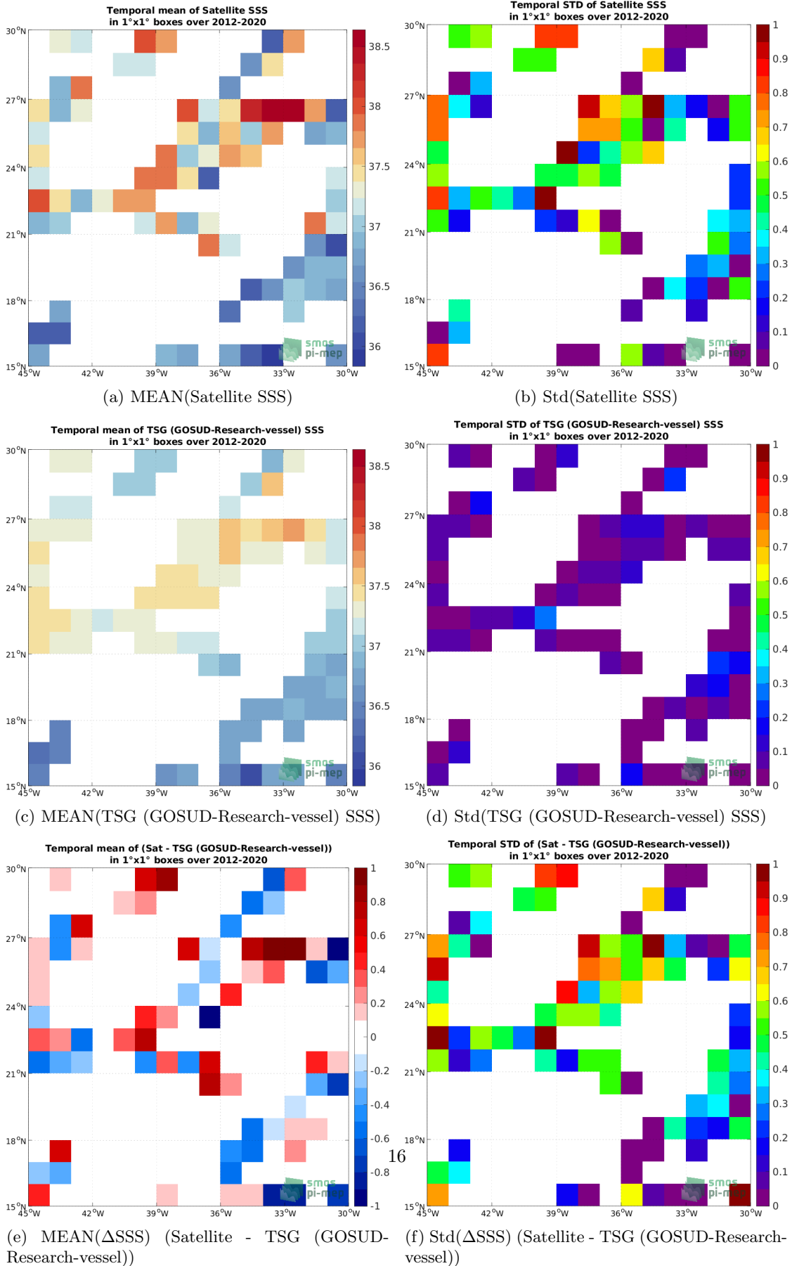
Figure 6: Temporal mean (left) and Std (right) of SSS from SMOS SSS L2Q v331 - 0.25 Deg (CATDS-CPDC) (top), TSG (GOSUD-Research-vessel) (middle), and of \Delta SSS (Satellite - TSG (GOSUD-Research-vessel)). Only match-up pairs are used to generate these maps.
