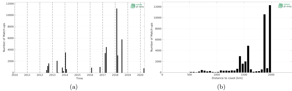
Figure 1: Number of match-ups between TSG (GOSUD-Research-vessel) and SMOS SSS L2Q v331 - 0.25 Deg (CATDS-CPDC) SSS as a function of time (a) and as function of the distance to coast (b) over the SPURS 1 Pi-MEP region and for the full satellite product period.
