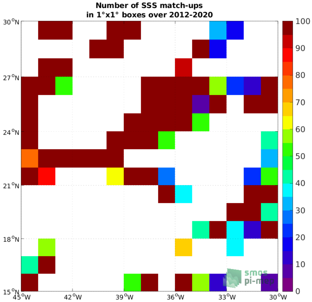
Figure 4: Number of SSS match-ups between TSG (GOSUD-Research-vessel) SSS and the SMOS SSS L2Q v331 - 0.25 Deg (CATDS-CPDC) SSS product for the SPURS 1 Pi-MEP region over 1^\circ \times 1^\circ boxes and for the full satellite product period.
