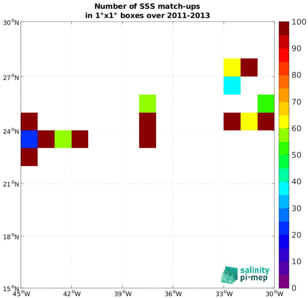
Figure 4: Number of SSS match-ups between TSG (CSIC-UTM) SSS and the SMOS SSS L2Q v331 - 0.25 Deg (CATDS-CPDC) SSS product for the SPURS 1 Pi-MEP region over 1°x1° boxes and for the full satellite product period.
