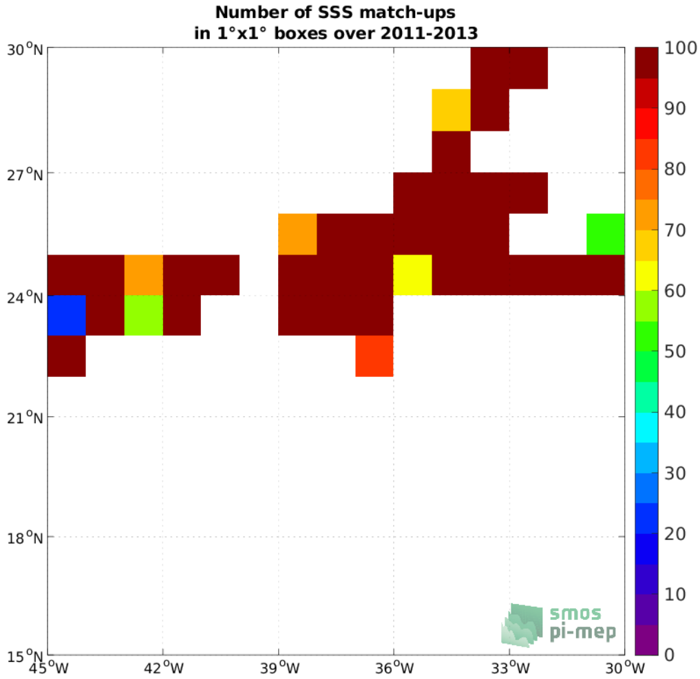
Figure 4: Number of SSS match-ups between TSG (CSIC-UTM) SSS and the SMOS SSS L2Q v331 - 0.25 Deg (CATDS-CPDC) SSS product for the SPURS 1 Pi-MEP region over 1^\circ \times 1^\circ boxes and for the full satellite product period.
