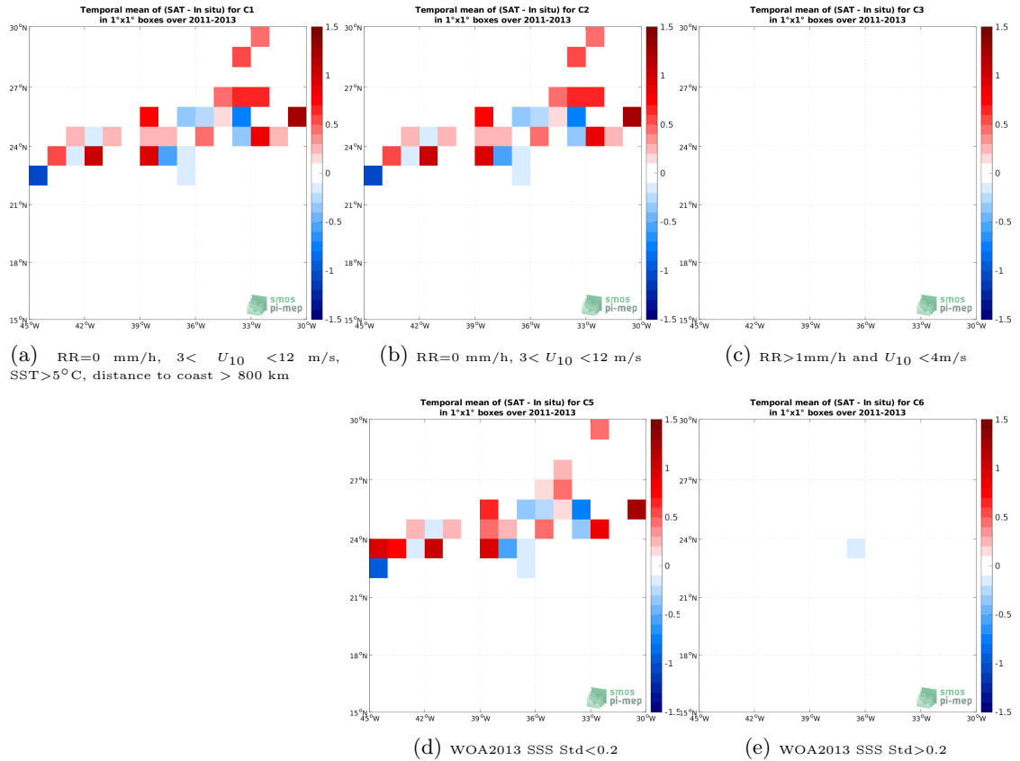
Figure 12: Temporal mean gridded over spatial boxes of size 1^{\circ}\times 1^{\circ} of \Delta\text{SSS} (SMOS SSS L2Q v331 - 0.25 Deg (CATDS-CPDC) - TSG (CSIC-UTM)) for 5 different subdatasets corresponding to:RR=0 mm/h, 3 < U_{10} < 12 m/s, SST >5^{\circ}\text{C} , distance to coast > 800 km (a), RR=0 mm/h, 3 < U_{10} < 12 m/s (b), RR >1 mm/h and U_{10} < 4 m/s (c), WOA2013 SSS Std <0.2 (d), WOA2013 SSS Std >0.2 (e).
