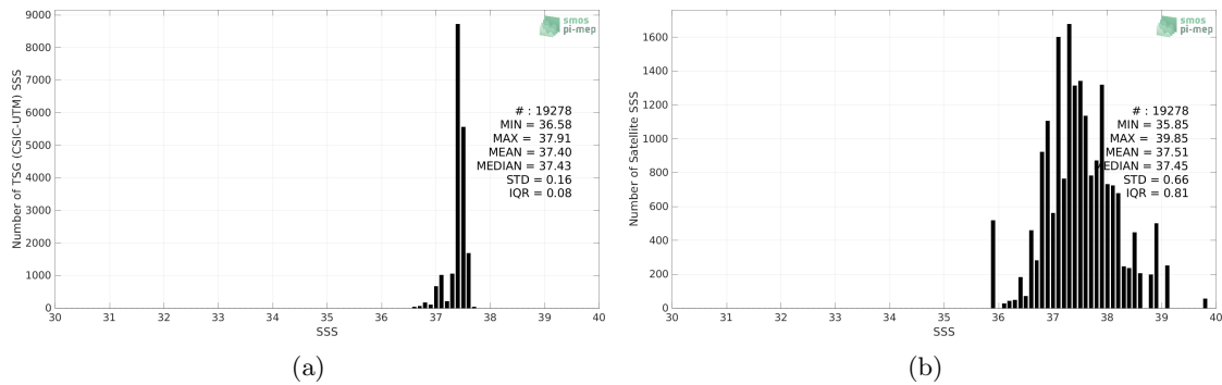
Figure 2: Histograms of SSS from TSG (CSIC-UTM) (a) and SMOS SSS L2Q v331 - 0.25 Deg (CATDS-CPDC) (b) considering all match-up pairs per bins of 0.1 over the SPURS 1 Pi-MEP region and for the full satellite product period.
