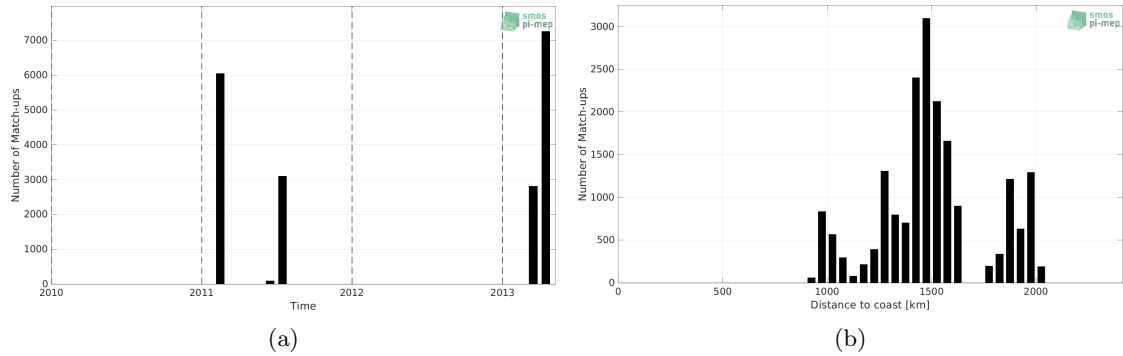
Figure 1: Number of match-ups between TSG (CSIC-UTM) and SMOS SSS L2Q v331 - 0.25 Deg (CATDS-CPDC) SSS as a function of time (a) and as function of the distance to coast (b) over the SPURS 1 Pi-MEP region and for the full satellite product period.
