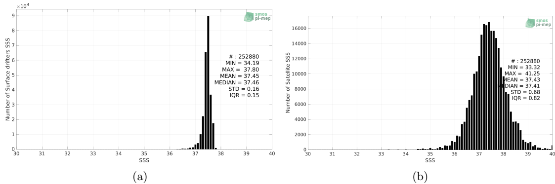
Figure 2: Histograms of SSS from Surface drifters (a) and SMOS SSS L2Q v331 - 0.25 Deg (CATDS-CPDC) (b) considering all match-up pairs per bins of 0.1 over the SPURS 1 Pi-MEP region and for the full satellite product period.
