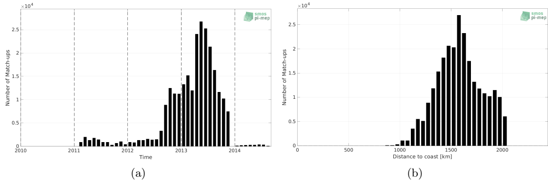
Figure 1: Number of match-ups between Surface drifters and SMOS SSS L2Q v331 - 0.25 Deg (CATDS-CPDC) SSS as a function of time (a) and as function of the distance to coast (b) over the SPURS 1 Pi-MEP region and for the full satellite product period.
