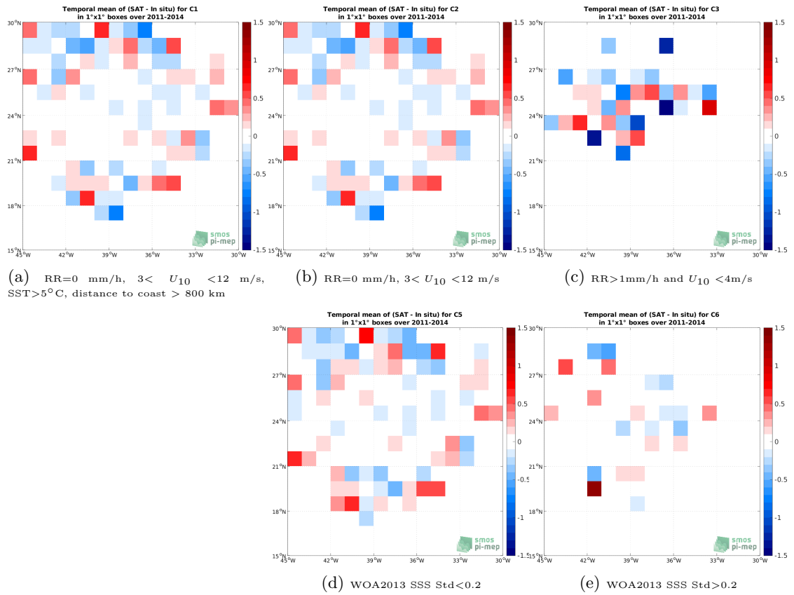
Figure 11: Temporal mean gridded over spatial boxes of size 1^\circ \times 1^\circ of \Delta SSS (SMOS SSS L2Q v331 - 0.25 Deg (CATDS-CPDC) - Surface drifters) for 5 different subdatasets corresponding to:RR=0 mm/h, 3 < U_{10} < 12 m/s, SST >5^\circ C, distance to coast > 800 km (a), RR=0 mm/h, 3 < U_{10} < 12 m/s (b), RR >1 mm/h and U_{10} < 4 m/s (c), WOA2013 SSS Std <0.2 (d), WOA2013 SSS Std >0.2 (e).
