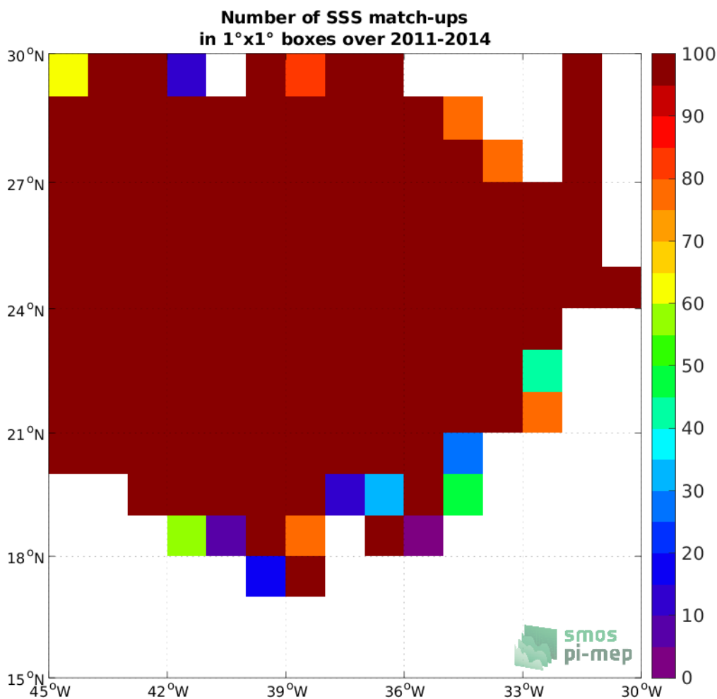
Figure 3: Number of SSS match-ups between Surface drifters SSS and the SMOS SSS L2Q v331 - 0.25 Deg (CATDS-CPDC) SSS product for the SPURS 1 Pi-MEP region over 1°x1° boxes and for the full satellite product period.
