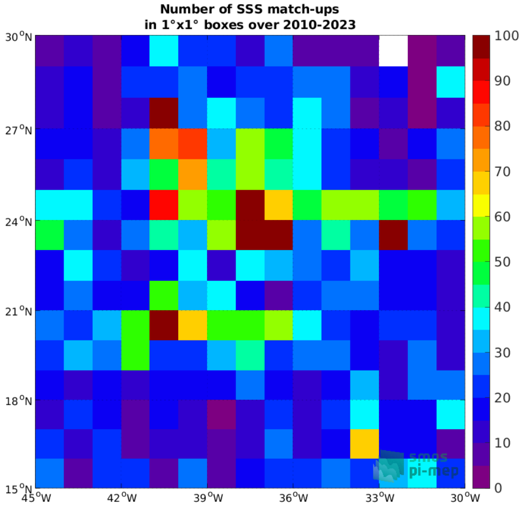
Figure 4: Number of SSS match-ups between Argo SSS and the SMOS SSS L2Q v331 - 0.25 Deg (CATDS-CPDC) SSS product for the SPURS 1 Pi-MEP region over 1°x1° boxes and for the full satellite product period.
