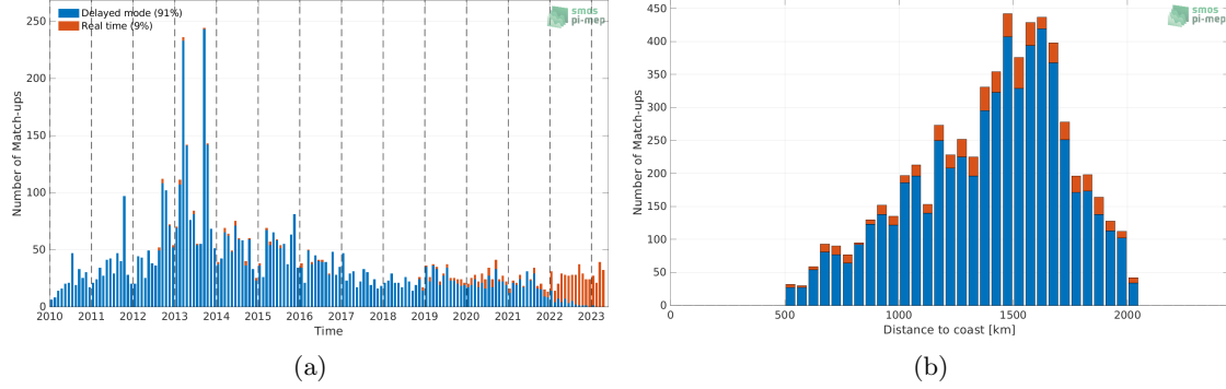
Figure 1: Number of match-ups between Argo and SMOS SSS L2Q v331 - 0.25 Deg (CATDS-CPDC) SSS as a function of time (a) and as function of the distance to coast (b) over the SPURS 1 Pi-MEP region and for the full satellite product period.
