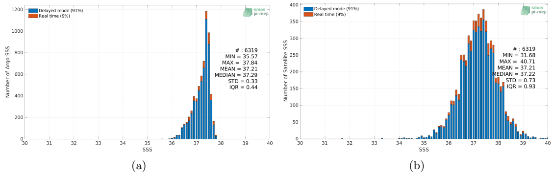
Figure 2: Histograms of SSS from Argo (a) and SMOS SSS L2Q v331 - 0.25 Deg (CATDS-CPDC) (b) considering all match-up pairs per bins of 0.1 over the SPURS 1 Pi-MEP region and for the full satellite product period.
