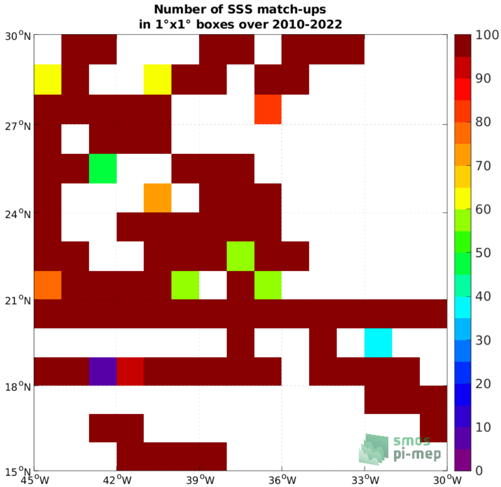
Figure 4: Number of SSS match-ups between TSG (SAMOS) SSS and the SMOS SSS L2Q v330 - 0.25 Deg (CATDS-CPDC) SSS product for the SPURS 1 Pi-MEP region over 1^\circ \times 1^\circ boxes and for the full satellite product period.
