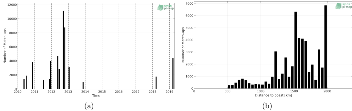
Figure 1: Number of match-ups between TSG (SAMOS) and SMOS SSS L2Q v330 - 0.25 Deg (CATDS-CPDC) SSS as a function of time (a) and as function of the distance to coast (b) over the SPURS 1 Pi-MEP region and for the full satellite product period.
