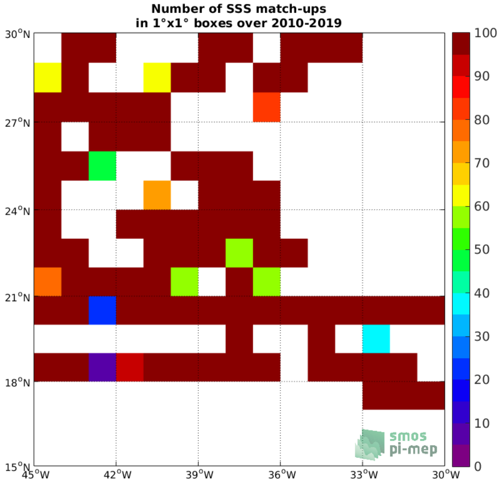
Figure 4: Number of SSS match-ups between TSG (SAMOS) SSS and the SMOS SSS L2Q v330 - 0.25 Deg (CATDS-CPDC) SSS product for the SPURS 1 Pi-MEP region over 1°x1° boxes and for the full satellite product period.
