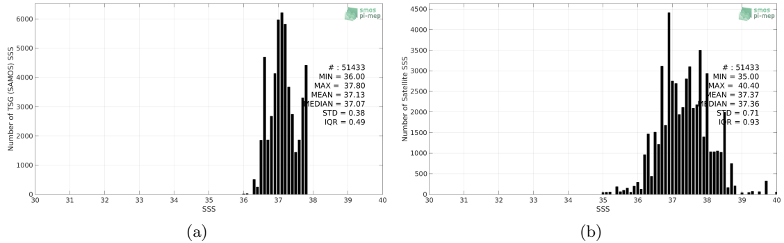
Figure 2: Histograms of SSS from TSG (SAMOS) (a) and SMOS SSS L2Q v330 - 0.25 Deg (CATDS-CPDC) (b) considering all match-up pairs per bins of 0.1 over the SPURS 1 Pi-MEP region and for the full satellite product period.
