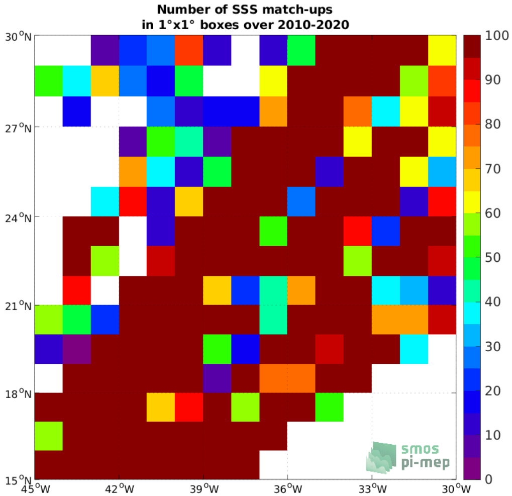
Figure 4: Number of SSS match-ups between TSG (LEGOS-DM) SSS and the SMOS SSS L2Q v330 - 0.25 Deg (CATDS-CPDC) SSS product for the SPURS 1 Pi-MEP region over 1°x1° boxes and for the full satellite product period.
