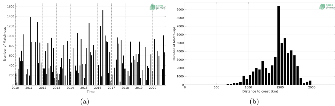
Figure 1: Number of match-ups between TSG (LEGOS-DM) and SMOS SSS L2Q v330 - 0.25 Deg (CATDS-CPDC) SSS as a function of time (a) and as function of the distance to coast (b) over the SPURS 1 Pi-MEP region and for the full satellite product period.
