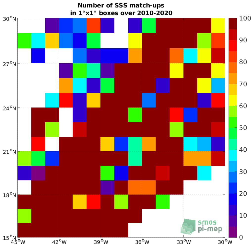
Figure 4: Number of SSS match-ups between TSG (LEGOS-DM) SSS and the SMOS SSS L2Q v330 - 0.25 Deg (CATDS-CPDC) SSS product for the SPURS 1 Pi-MEP region over 1^\circ \times 1^\circ boxes and for the full satellite product period.
