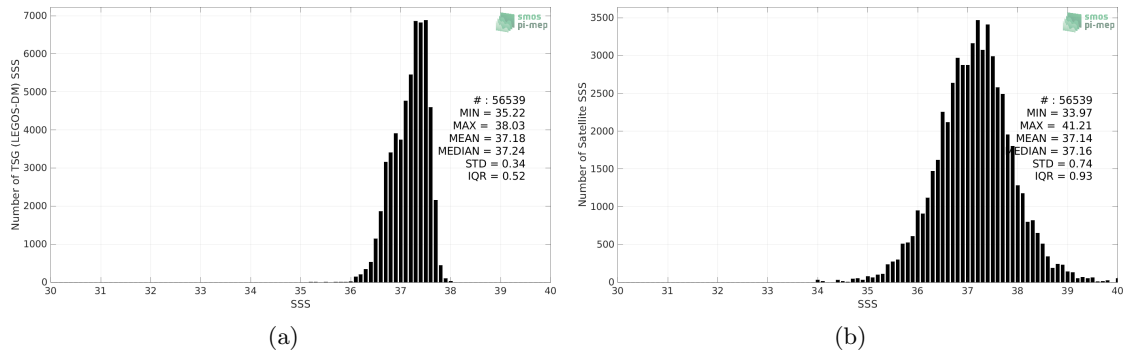
Figure 2: Histograms of SSS from TSG (LEGOS-DM) (a) and SMOS SSS L2Q v330 - 0.25 Deg (CATDS-CPDC) (b) considering all match-up pairs per bins of 0.1 over the SPURS 1 Pi-MEP region and for the full satellite product period.
