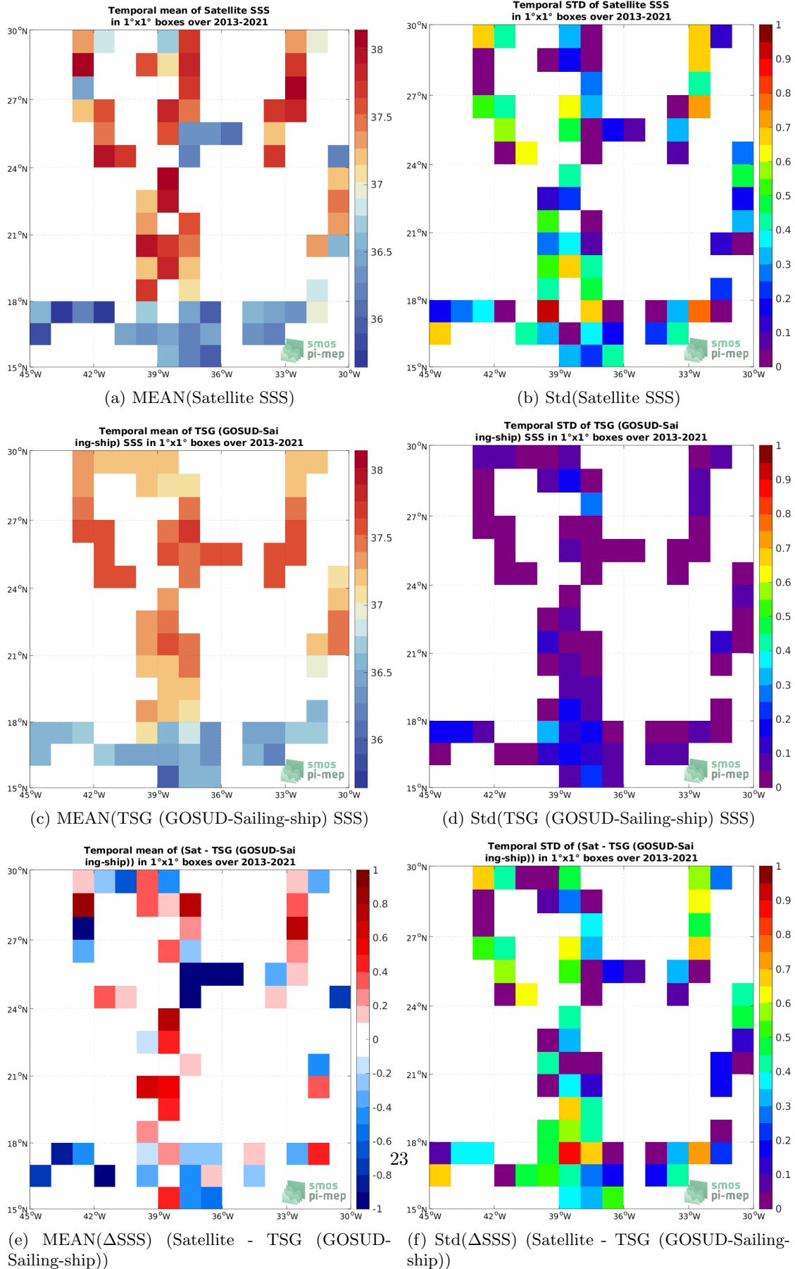
Figure 6: Temporal mean (left) and Std (right) of SSS from SMOS SSS L2Q v330 - 0.25 Deg (CATDS-CPDC) (top), TSG (GOSUD-Sailing-ship) (middle), and of \Delta SSS (Satellite - TSG (GOSUD-Sailing-ship)). Only match-up pairs are used to generate these maps.
