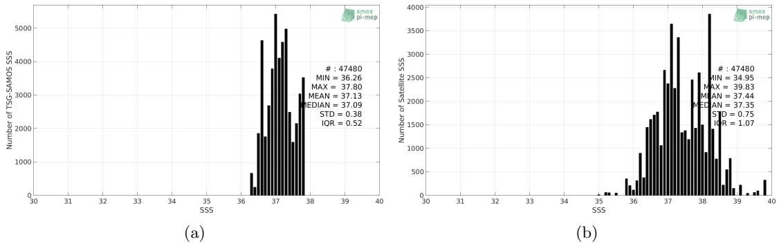
Figure 2: Histograms of SSS from TSG-SAMOS (a) and SMOS L2Q v321 - 0.25 Deg (CATDS-CPDC) (b) considering all match-up pairs per bins of 0.1 over the SPURS 1 Pi-MEP region and for the full satellite product period.
