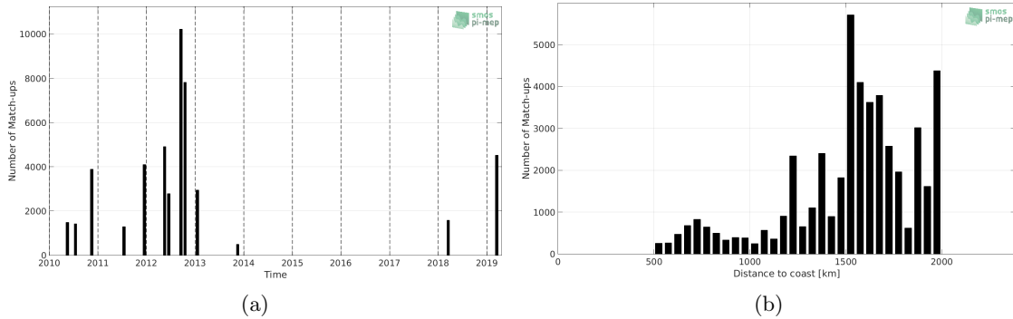
Figure 1: Number of match-ups between TSG-SAMOS and SMOS L2Q v321 - 0.25 Deg (CATDS-CPDC) SSS as a function of time (a) and as function of the distance to coast (b) over the SPURS 1 Pi-MEP region and for the full satellite product period.
