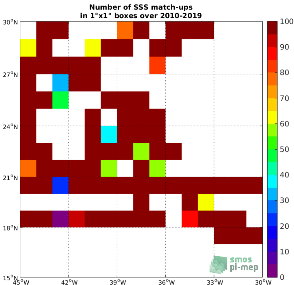
Figure 4: Number of SSS match-ups between TSG-SAMOS SSS and the SMOS L2Q v321 - 0.25 Deg (CATDS-CPDC) SSS product for the SPURS 1 Pi-MEP region over 1°x1° boxes and for the full satellite product period.
