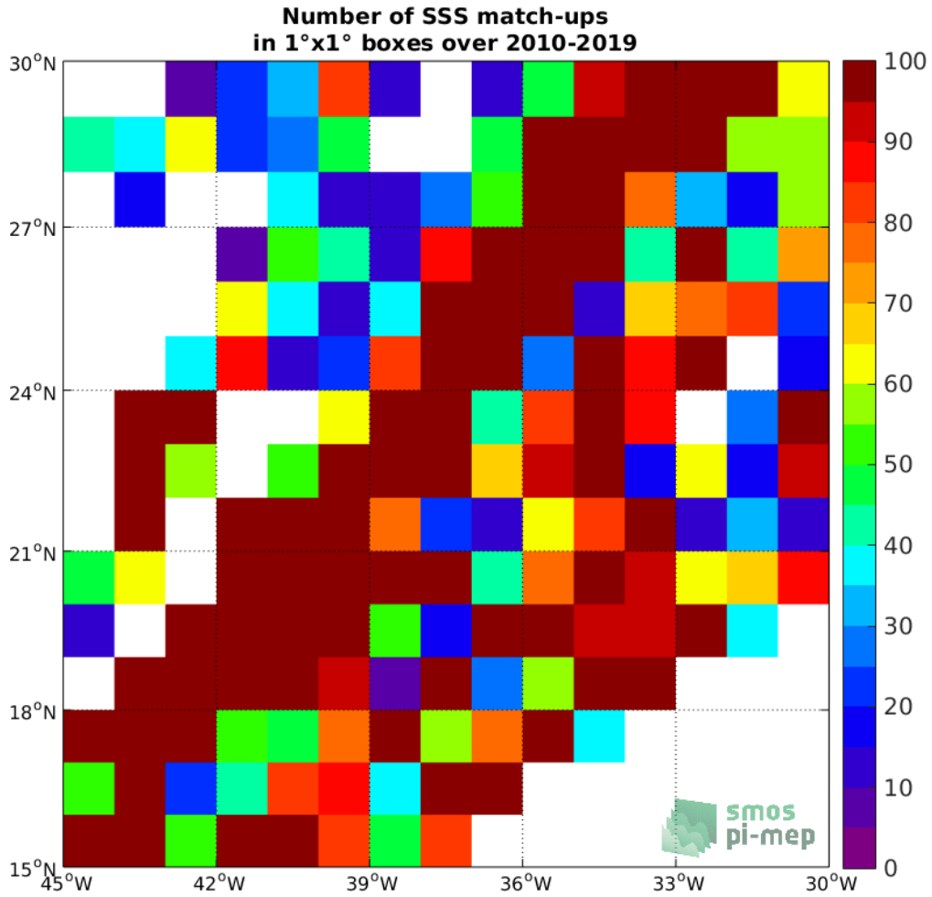
Figure 4: Number of SSS match-ups between TSG (LEGOS-DM) SSS and the SMOS SSS L2Q v321 - 0.25 Deg (CATDS-CPDC) SSS product for the SPURS 1 Pi-MEP region over 1^\circ \times 1^\circ boxes and for the full satellite product period.
