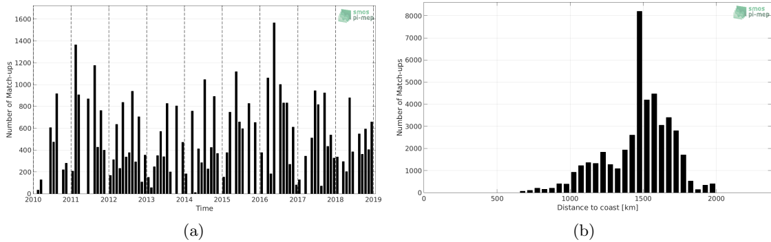
Figure 1: Number of match-ups between TSG-LEGOS-DM and SMOS L2Q v321 - 0.25 Deg (CATDS-CPDC) SSS as a function of time (a) and as function of the distance to coast (b) over the SPURS 1 Pi-MEP region and for the full satellite product period.
