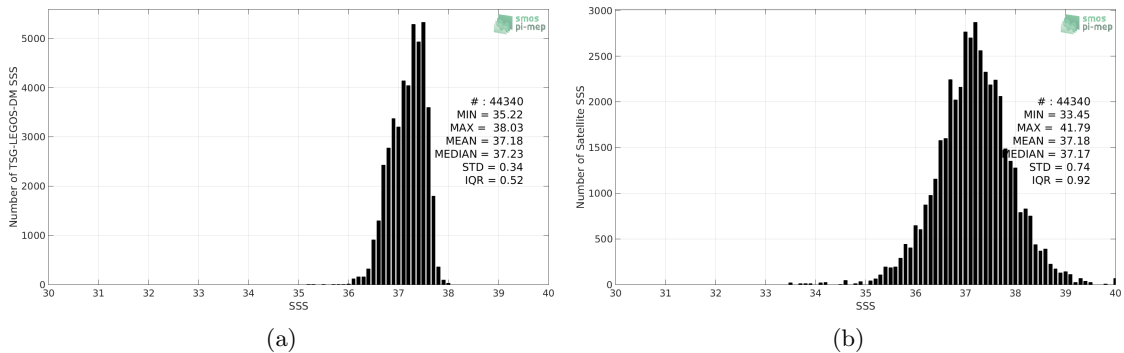
Figure 2: Histograms of SSS from TSG-LEGOS-DM (a) and SMOS L2Q v321 - 0.25 Deg (CATDS-CPDC) (b) considering all match-up pairs per bins of 0.1 over the SPURS 1 Pi-MEP region and for the full satellite product period.
