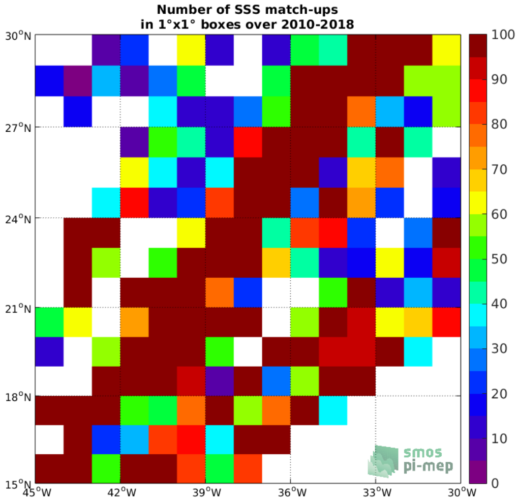
Figure 4: Number of SSS match-ups between TSG-LEGOS-DM SSS and the SMOS L2Q v321 - 0.25 Deg (CATDS-CPDC) SSS product for the SPURS 1 Pi-MEP region over 1°x1° boxes and for the full satellite product period.
