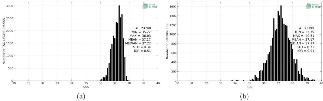
Figure 2: Histograms of SSS from TSG-LEGOS-DM (a) and SMOS-L3-CATDS-CPDC-V321-L2Q (b) considering all match-up pairs per bins of 0.1 over the SPURS 1 Pi-MEP region and for the full satellite product period.
