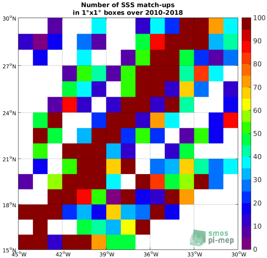
Figure 4: Number of SSS match-ups between TSG-LEGOS-DM SSS and the SMOS-L3-CATDS-CPDC-V321-L2Q SSS product for the SPURS 1 Pi-MEP region over 1°x1° boxes and for the full satellite product period.
