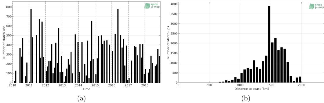
Figure 1: Number of match-ups between TSG-LEGOS-DM and SMOS-L3-CATDS-CPDC-V321-L2Q SSS as a function of time (a) and as function of the distance to coast (b) over the SPURS 1 Pi-MEP region and for the full satellite product period.
