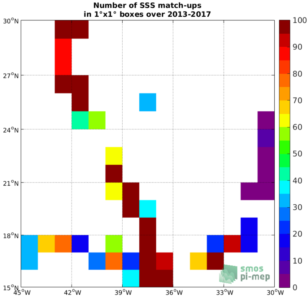
Figure 4: Number of SSS match-ups between TSG (GOSUD-Sailing-ship) SSS and the SMOS SSS L2Q v321 - 0.25 Deg (CATDS-CPDC) SSS product for the SPURS 1 Pi-MEP region over 1^\circ \times 1^\circ boxes and for the full satellite product period.
