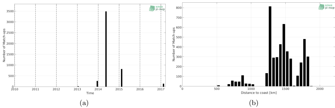
Figure 1: Number of match-ups between TSG (GOSUD-Sailing-ship) and SMOS SSS L2Q v321 - 0.25 Deg (CATDS-CPDC) SSS as a function of time (a) and as function of the distance to coast (b) over the SPURS 1 Pi-MEP region and for the full satellite product period.
