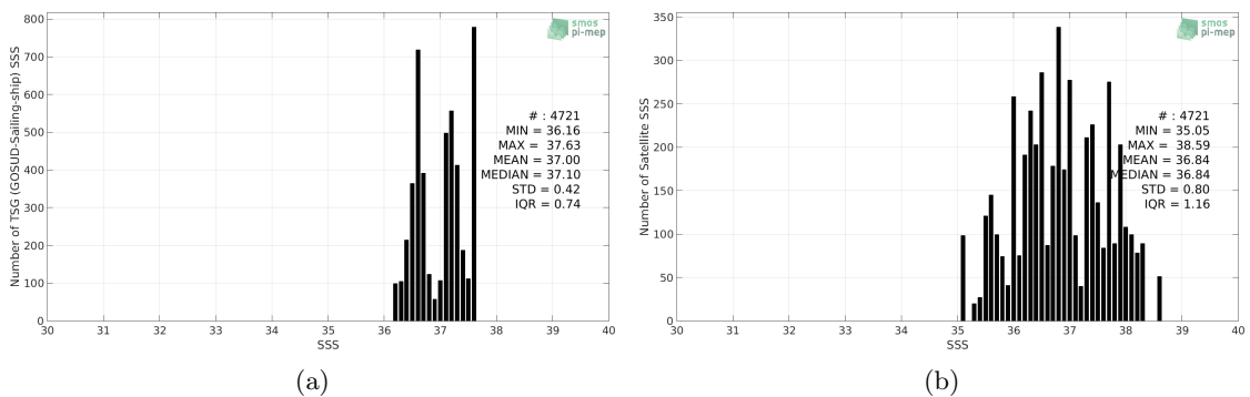
Figure 2: Histograms of SSS from TSG (GOSUD-Sailing-ship) (a) and SMOS SSS L2Q v321 - 0.25 Deg (CATDS-CPDC) (b) considering all match-up pairs per bins of 0.1 over the SPURS 1 Pi-MEP region and for the full satellite product period.
