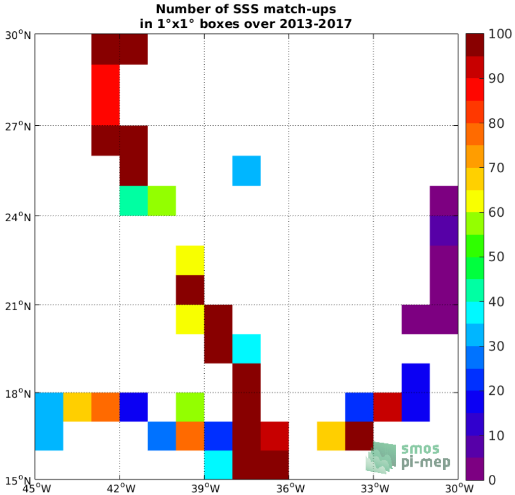
Figure 4: Number of SSS match-ups between TSG (GOSUD-Sailing-ship) SSS and the SMOS SSS L2Q v321 - 0.25 Deg (CATDS-CPDC) SSS product for the SPURS 1 Pi-MEP region over 1°x1° boxes and for the full satellite product period.
