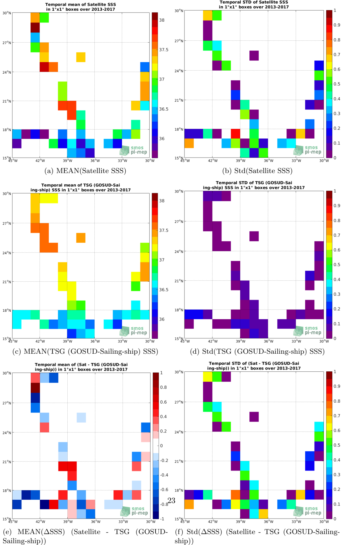
Figure 6: Temporal mean (left) and Std (right) of SSS from SMOS SSS L2Q v321 - 0.25 Deg (CATDS-CPDC) (top), TSG (GOSUD-Sailing-ship) (middle), and of \Delta SSS (Satellite - TSG (GOSUD-Sailing-ship)). Only match-up pairs are used to generate these maps.
