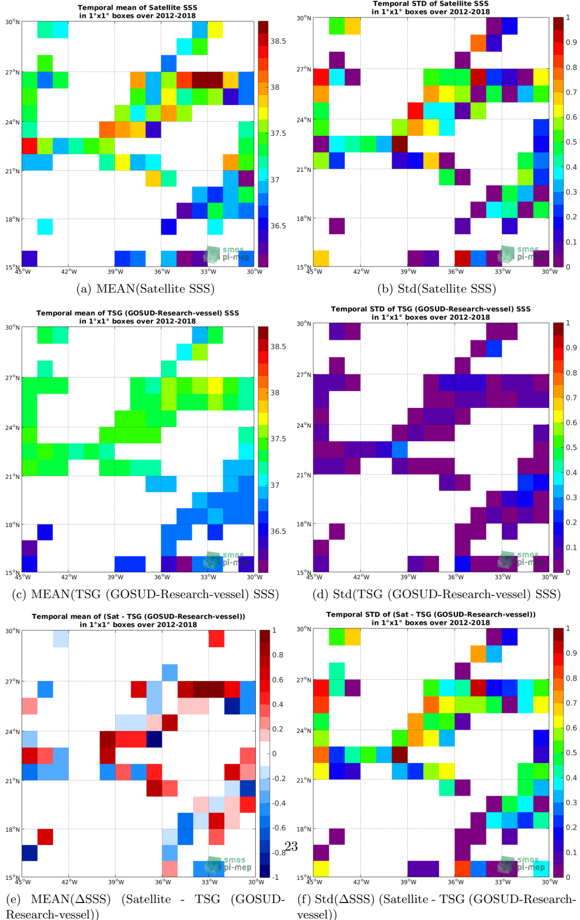
Figure 6: Temporal mean (left) and Std (right) of SSS from SMOS SSS L2Q v321 - 0.25 Deg (CATDS-CPDC) (top), TSG (GOSUD-Research-vessel) (middle), and of \Delta SSS (Satellite - TSG (GOSUD-Research-vessel)). Only match-up pairs are used to generate these maps.
