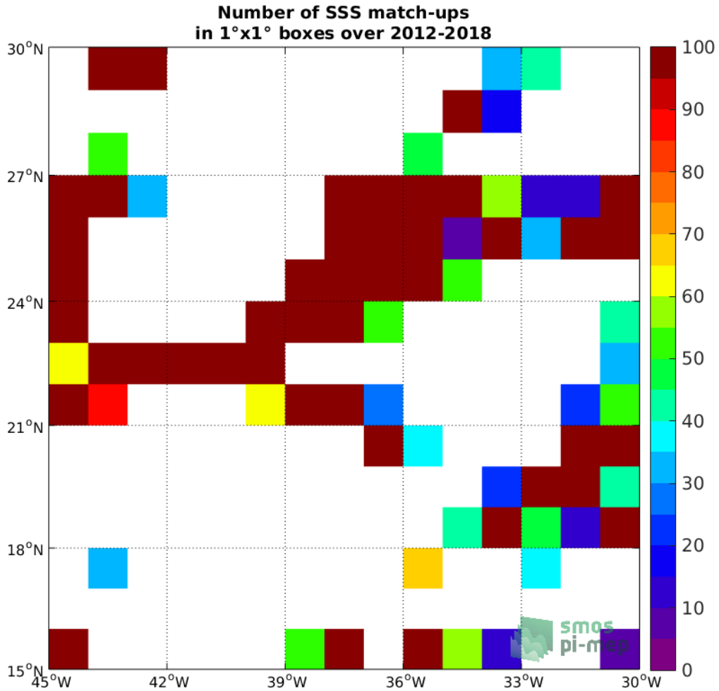
Figure 4: Number of SSS match-ups between TSG (GOSUD-Research-vessel) SSS and the SMOS SSS L2Q v321 - 0.25 Deg (CATDS-CPDC) SSS product for the SPURS 1 Pi-MEP region over 1°x1° boxes and for the full satellite product period.
