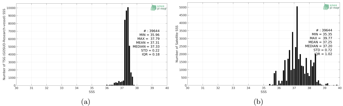
Figure 2: Histograms of SSS from TSG (GOSUD-Research-vessel) (a) and SMOS SSS L2Q v321 - 0.25 Deg (CATDS-CPDC) (b) considering all match-up pairs per bins of 0.1 over the SPURS 1 Pi-MEP region and for the full satellite product period.
