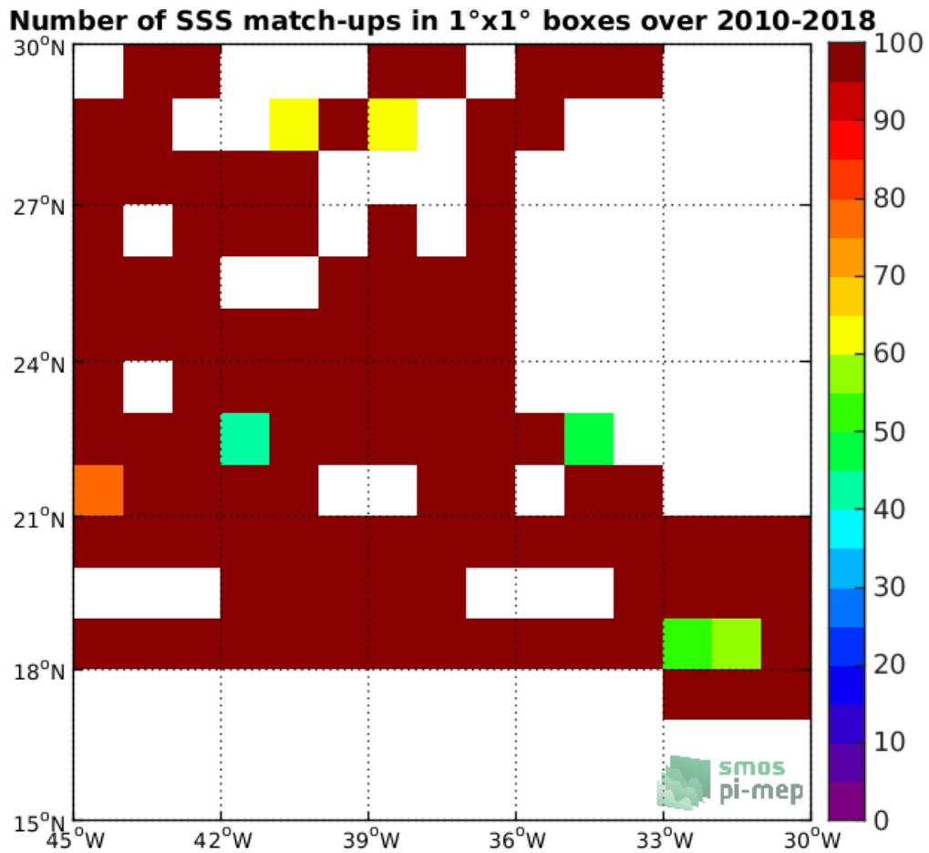
Figure 4: Number of SSS match-ups between TSG-SAMOS SSS and the SMOS-L3-CATDS-CPDC-V317-MONTHLY-25KM SSS product for the SPURS 1 Pi-MEP region over 1°x1° boxes and for the full satellite product period.
