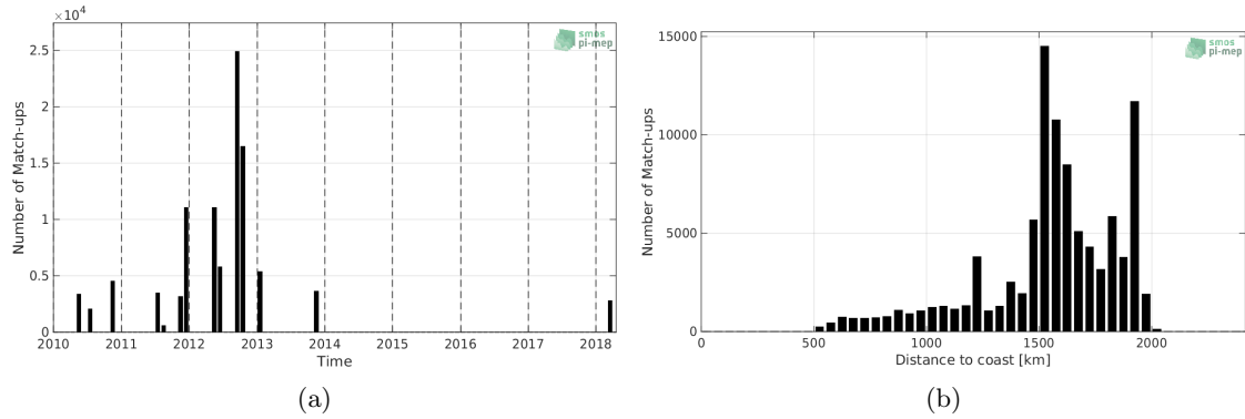
Figure 1: Number of match-ups between TSG-SAMOS and SMOS-L3-CATDS-CPDC-V317-MONTHLY-25KM SSS as a function of time (a) and as function of the distance to coast (b) over the SPURS 1 Pi-MEP region and for the full satellite product period.
