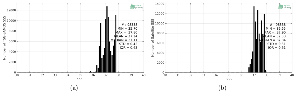
Figure 2: Histograms of SSS from TSG-SAMOS (a) and SMOS-L3-CATDS-CPDC-V317-MONTHLY-25KM (b) considering all match-up pairs per bins of 0.1 over the SPURS 1 Pi-MEP region and for the full satellite product period.
