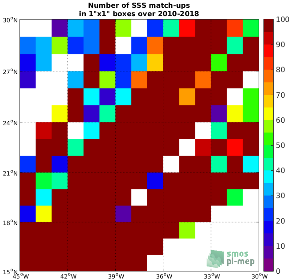
Figure 4: Number of SSS match-ups between TSG-LEGOS-DM SSS and the SMOS-L3-CATDS-CPDC-V317-MONTHLY-25KM SSS product for the SPURS 1 Pi-MEP region over 1°x1° boxes and for the full satellite product period.
