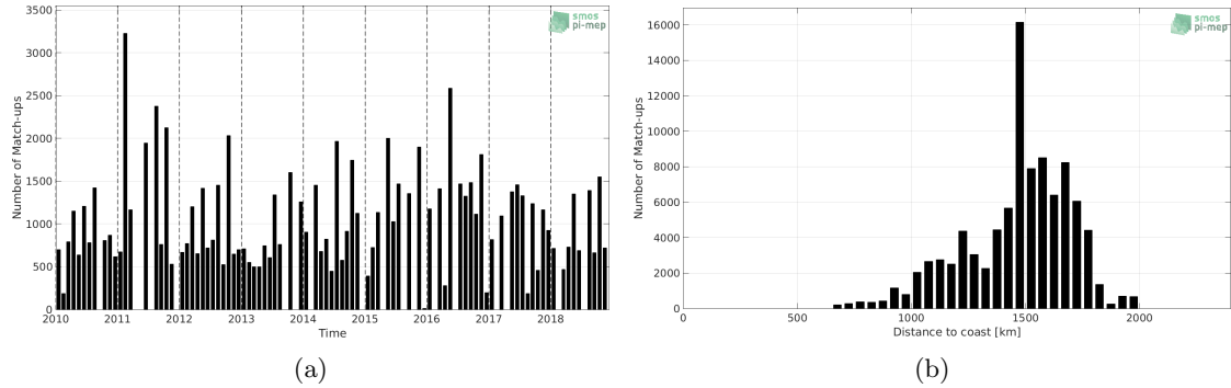
Figure 1: Number of match-ups between TSG-LEGOS-DM and SMOS-L3-CATDS-CPDC-V317-MONTHLY-25KM SSS as a function of time (a) and as function of the distance to coast (b) over the SPURS 1 Pi-MEP region and for the full satellite product period.
