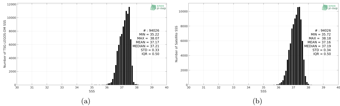
Figure 2: Histograms of SSS from TSG-LEGOS-DM (a) and SMOS-L3-CATDS-CPDC-V317-MONTHLY-25KM (b) considering all match-up pairs per bins of 0.1 over the SPURS 1 Pi-MEP region and for the full satellite product period.
