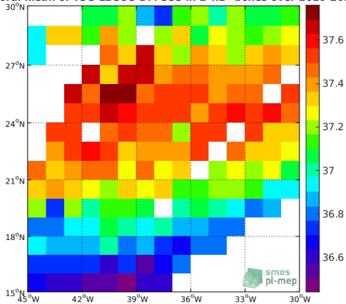
(c) MEAN(TSG-LEGOS-DM SSS)
