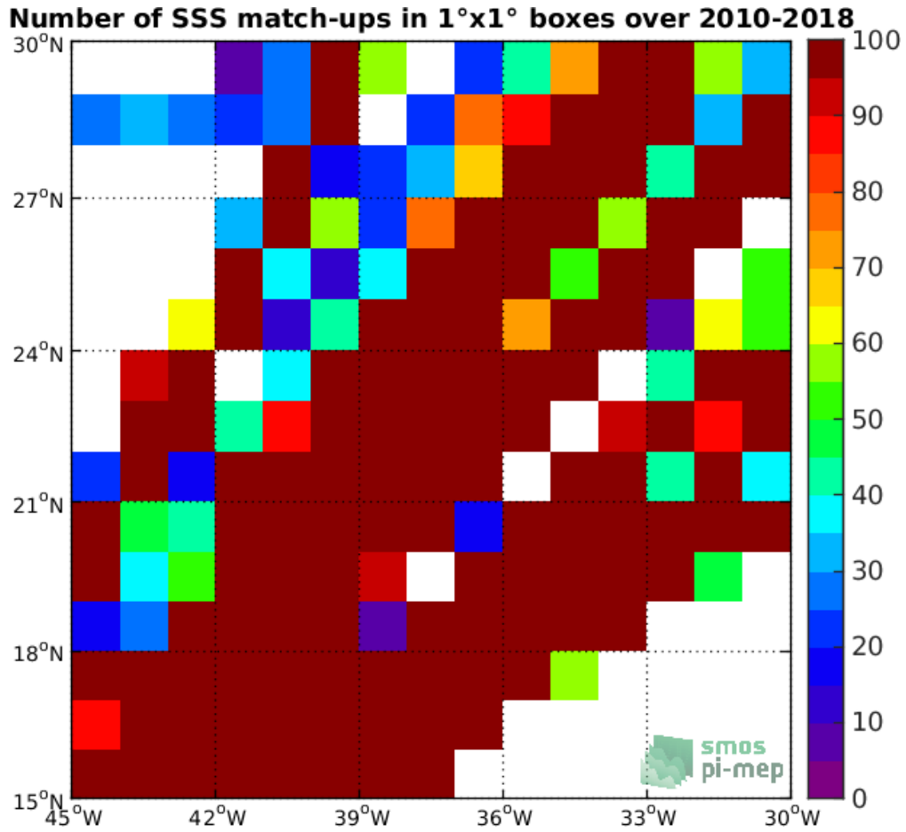
Figure 4: Number of SSS match-ups between TSG-LEGOS-DM SSS and the SMOS-L3-CATDS-CPDC-V317-MONTHLY-25KM SSS product for the SPURS 1 Pi-MEP region over 1°x1° boxes and for the full satellite product period.
