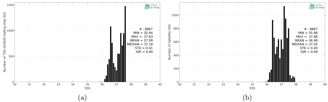
Figure 2: Histograms of SSS from TSG-GOSUD-Sailing-ship (a) and SMOS L3 v317 - Monthly - 25 km (CATDS-CPDC) (b) considering all match-up pairs per bins of 0.1 over the SPURS 1 Pi-MEP region and for the full satellite product period.
