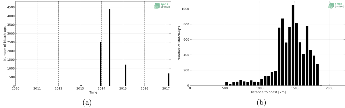
Figure 1: Number of match-ups between TSG-GOSUD-Sailing-ship and SMOS L3 v317 - Monthly - 25 km (CATDS-CPDC) SSS as a function of time (a) and as function of the distance to coast (b) over the SPURS 1 Pi-MEP region and for the full satellite product period.
