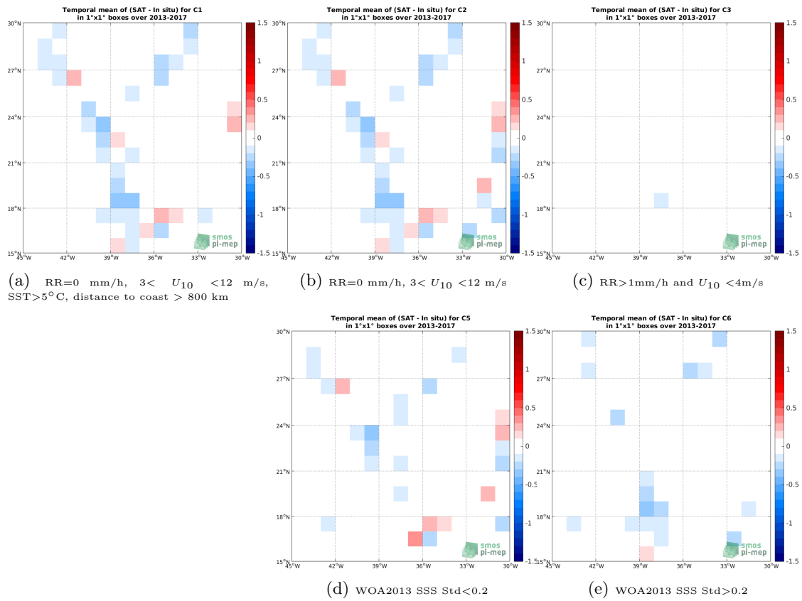
Figure 12: Temporal mean gridded over spatial boxes of size 1^\circ \times 1^\circ of \Delta SSS (SMOS L3 v317 - Monthly - 25 km (CATDS-CPDC) - TSG-GOSUD-Sailing-ship) for 5 different subdatasets corresponding to: RR=0 mm/h, 3 < U_{10} < 12 m/s, SST>5°C, distance to coast > 800 km (a), RR=0 mm/h, 3 < U_{10} < 12 m/s (b), RR>1mm/h and U_{10} < 4 m/s (c), WOA2013 SSS Std<0.2 (d), WOA2013 SSS Std>0.2 (e).
