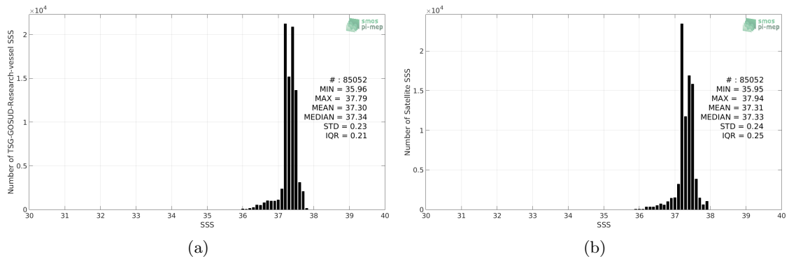
Figure 2: Histograms of SSS from TSG-GOSUD-Research-vessel (a) and SMOS-L3-CATDS-CPDC-V317-MONTHLY-25KM (b) considering all match-up pairs per bins of 0.1 over the SPURS 1 Pi-MEP region and for the full satellite product period.
