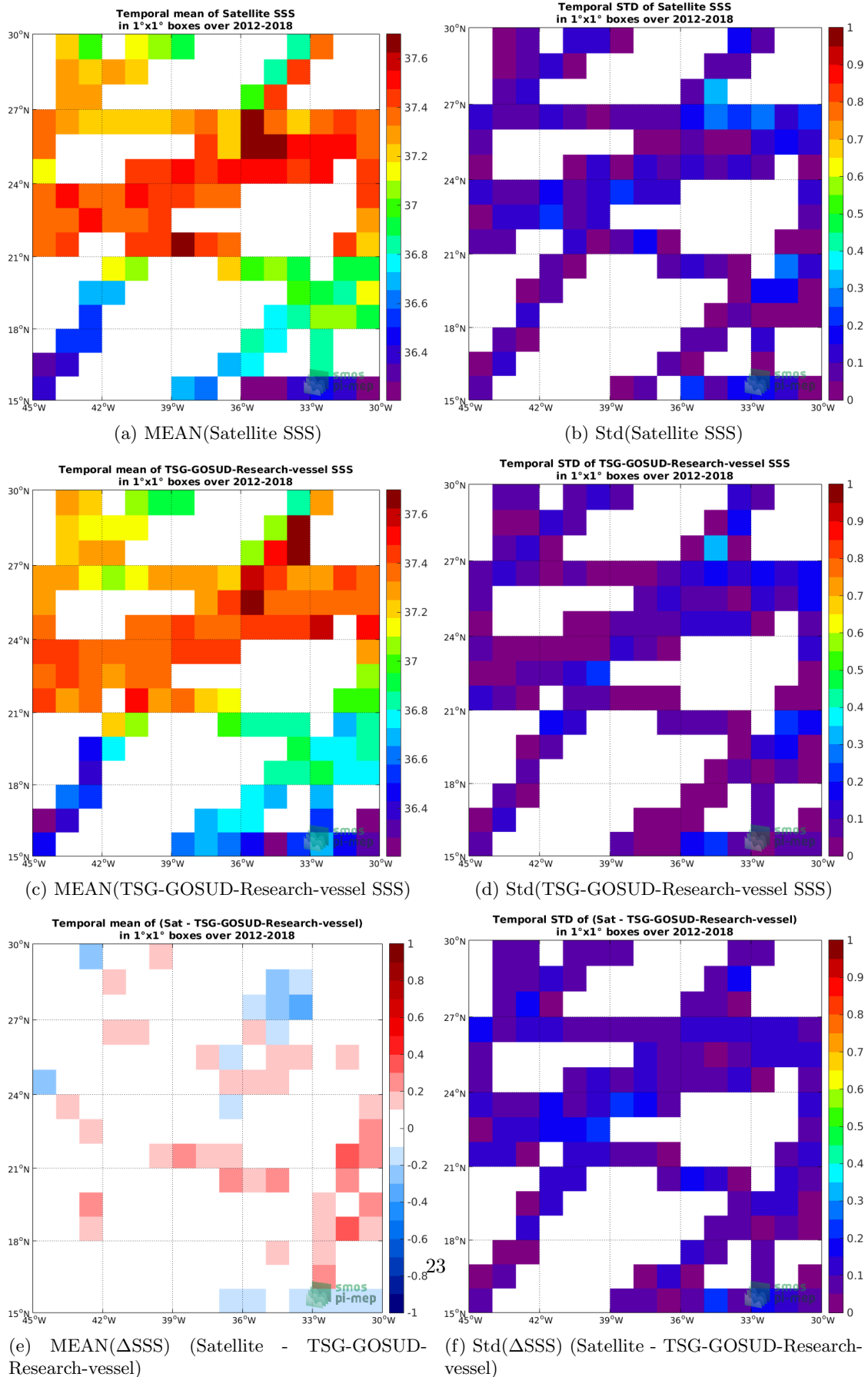
Figure 6: Temporal mean (left) and Std (right) of SSS from SMOS-L3-CATDS-CPDC-V317-MONTHLY-25KM (top), TSG-GOSUD-Research-vessel (middle), and of \Delta SSS (Satellite - TSG-GOSUD-Research-vessel). Only match-up pairs are used to generate these maps.
