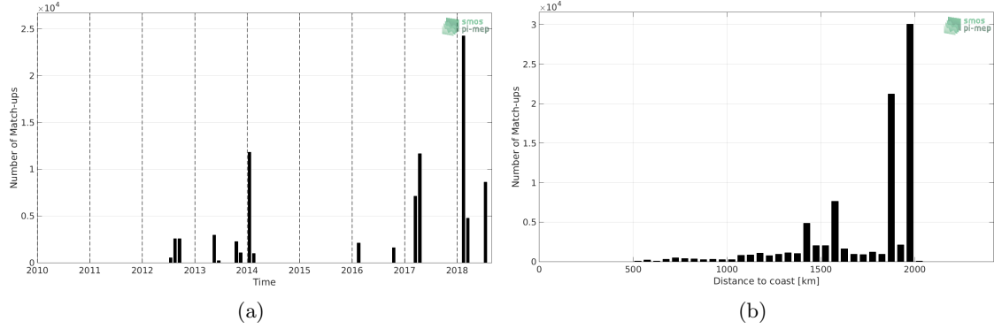
Figure 1: Number of match-ups between TSG-GOSUD-Research-vessel and SMOS-L3-CATDS-CPDC-V317-MONTHLY-25KM SSS as a function of time (a) and as function of the distance to coast (b) over the SPURS 1 Pi-MEP region and for the full satellite product period.
