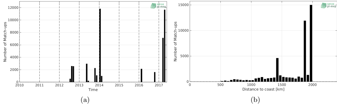
Figure 1: Number of match-ups between TSG-GOSUD-Research-vessel and SMOS-L3-CATDS-CPDC-V317-MONTHLY-25KM SSS as a function of time (a) and as function of the distance to coast (b) over the SPURS 1 Pi-MEP region and for the full satellite product period.
