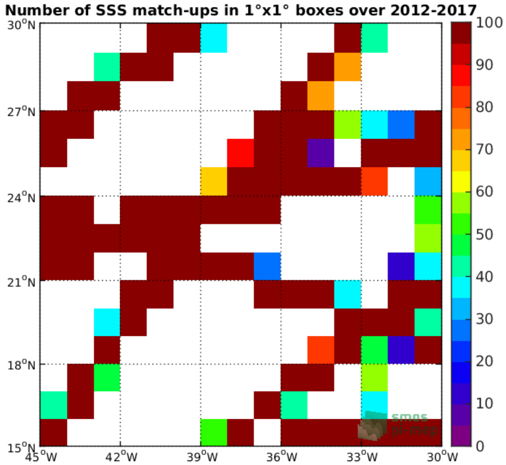
Figure 4: Number of SSS match-ups between TSG-GOSUD-Research-vessel SSS and the SMOS-L3-CATDS-CPDC-V317-MONTHLY-25KM SSS product for the SPURS 1 Pi-MEP region over 1°x1° boxes and for the full satellite product period.
