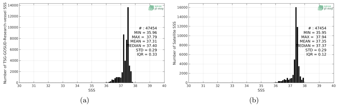
Figure 2: Histograms of SSS from TSG-GOSUD-Research-vessel (a) and SMOS-L3-CATDS-CPDC-V317-MONTHLY-25KM (b) considering all match-up pairs per bins of 0.1 over the SPURS 1 Pi-MEP region and for the full satellite product period.
