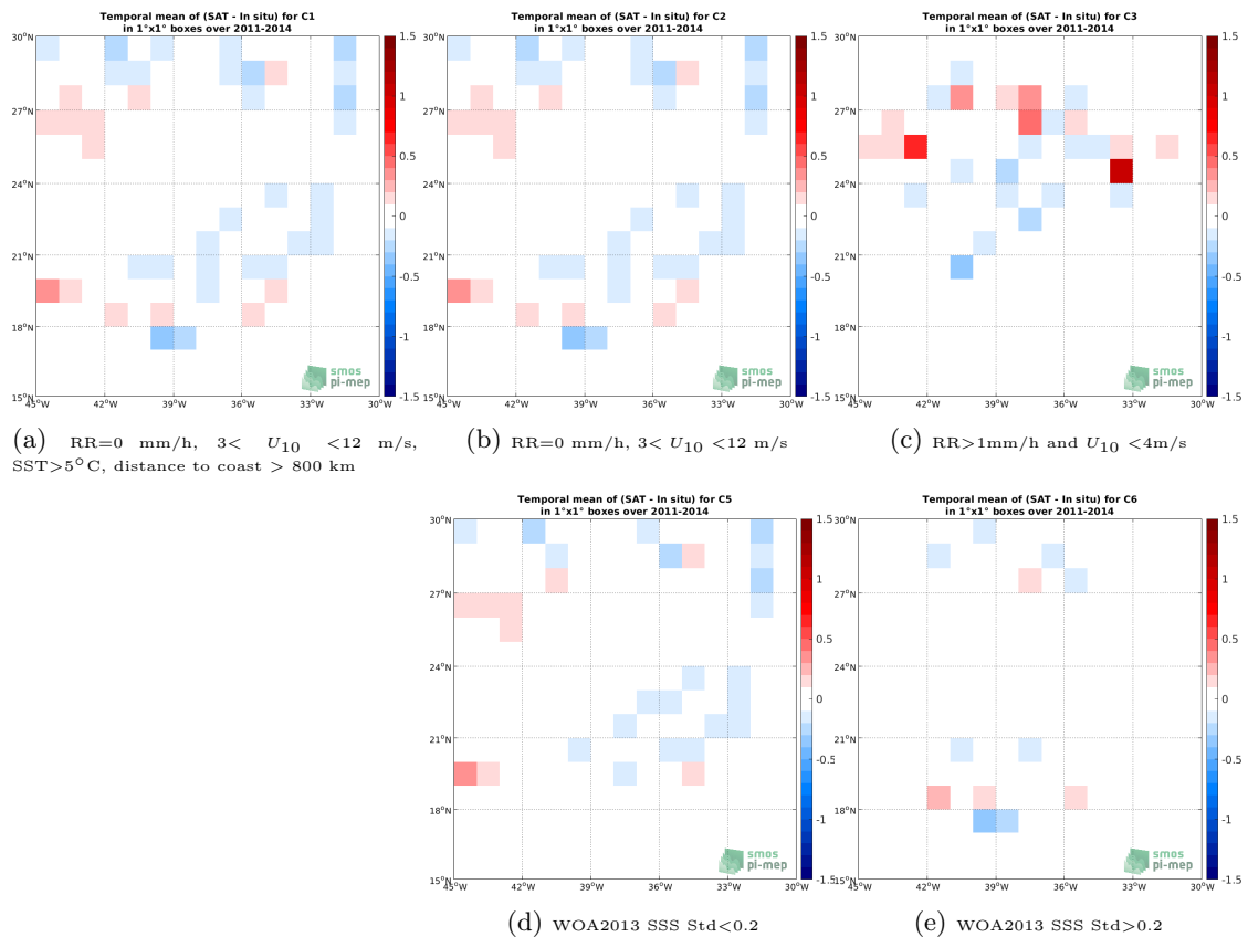
Figure 11: Temporal mean gridded over spatial boxes of size 1^\circ \times 1^\circ of \Delta\text{SSS} (SMOS SSS L3 v317 - Monthly - 25 km (CATDS-CPDC) - Surface drifters) for 5 different subdatasets corresponding to:RR=0 mm/h, 3 < U_{10} < 12 m/s, SST>5°C, distance to coast > 800 km (a), RR=0 mm/h, 3 < U_{10} < 12 m/s (b), RR>1mm/h and U_{10} < 4 m/s (c), WOA2013 SSS Std<0.2 (d), WOA2013 SSS Std>0.2 (e).
