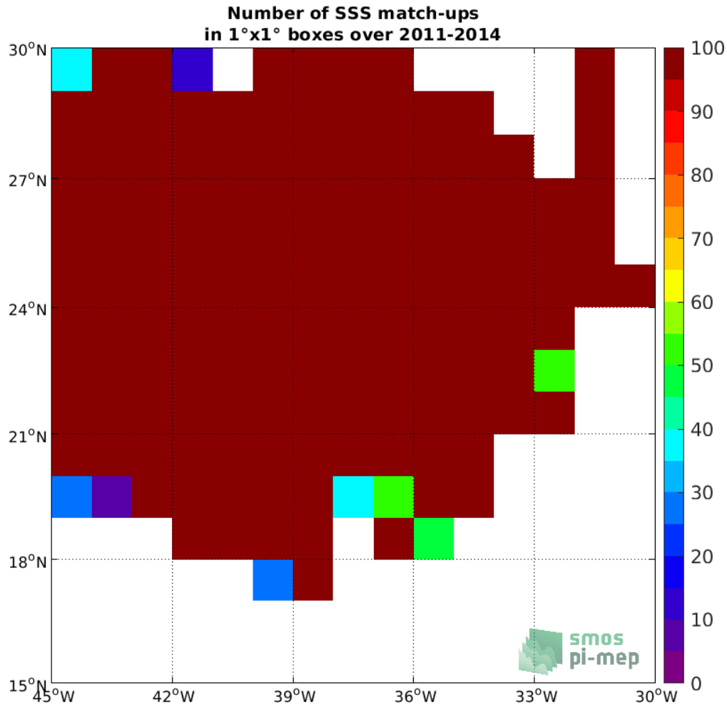
Figure 3: Number of SSS match-ups between Surface drifters SSS and the SMOS SSS L3 v317 - Monthly - 25 km (CATDS-CPDC) SSS product for the SPURS 1 Pi-MEP region over 1^\circ \times 1^\circ boxes and for the full satellite product period.
