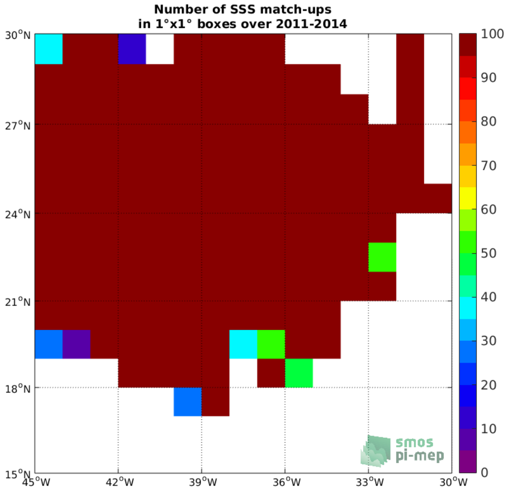
Figure 3: Number of SSS match-ups between Surface drifters SSS and the SMOS L3 v317 - Monthly - 25 km (CATDS-CPDC) SSS product for the SPURS 1 Pi-MEP region over 1°x1° boxes and for the full satellite product period.
