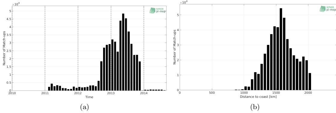
Figure 1: Number of match-ups between Surface drifters and SMOS L3 v317 - Monthly - 25 km (CATDS-CPDC) SSS as a function of time (a) and as function of the distance to coast (b) over the SPURS 1 Pi-MEP region and for the full satellite product period.
