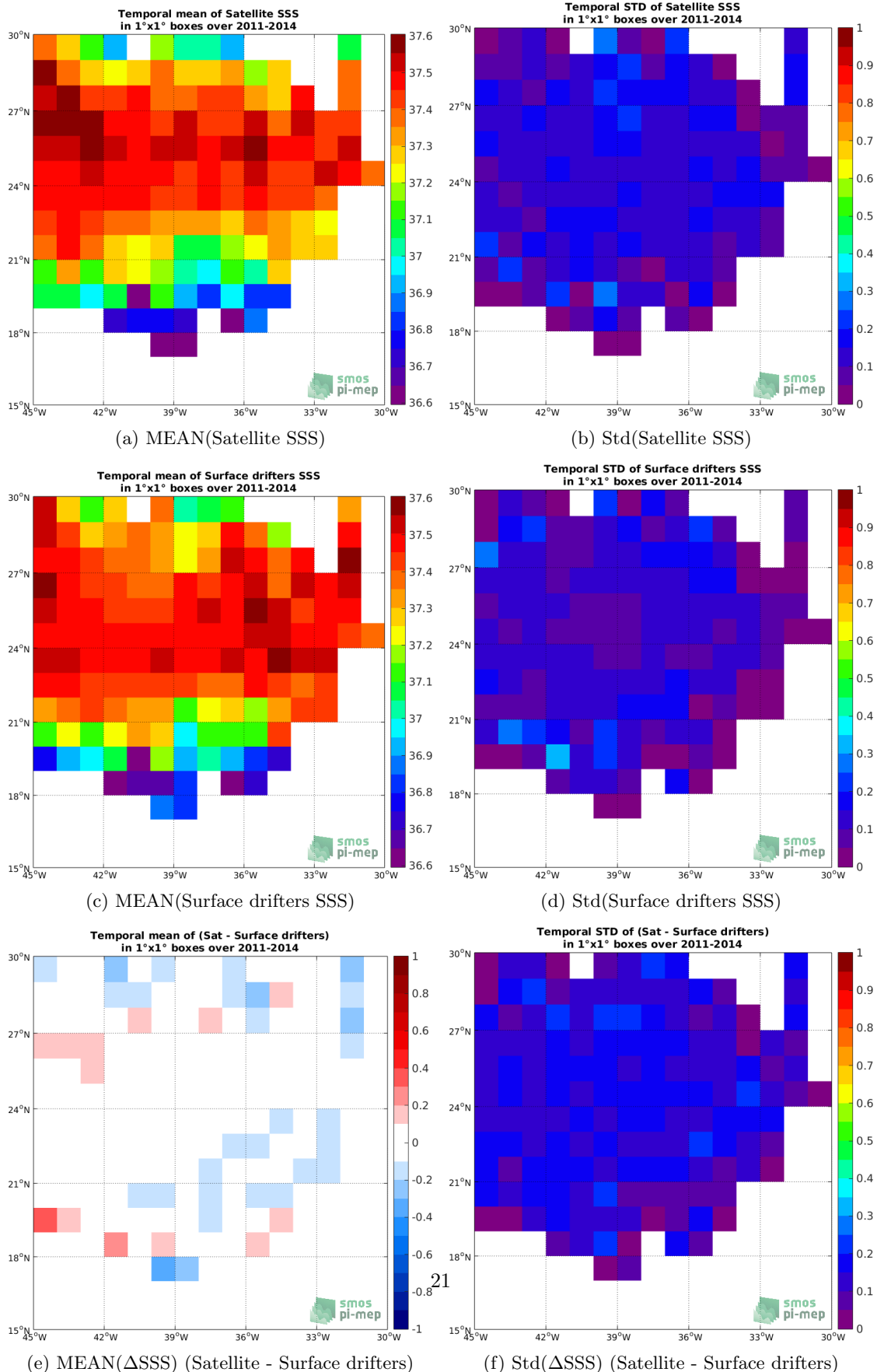
Figure 5: Temporal mean (left) and Std (right) of SSS from SMOS L3 v317 - Monthly - 25 km (CATDS-CPDC) (top), Surface drifters (middle), and of \Delta SSS (Satellite - Surface drifters). Only match-up pairs are used to generate these maps.
