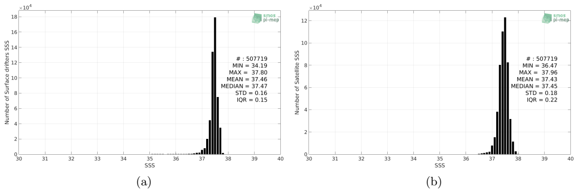
Figure 2: Histograms of SSS from Surface drifters (a) and SMOS L3 v317 - Monthly - 25 km (CATDS-CPDC) (b) considering all match-up pairs per bins of 0.1 over the SPURS 1 Pi-MEP region and for the full satellite product period.
