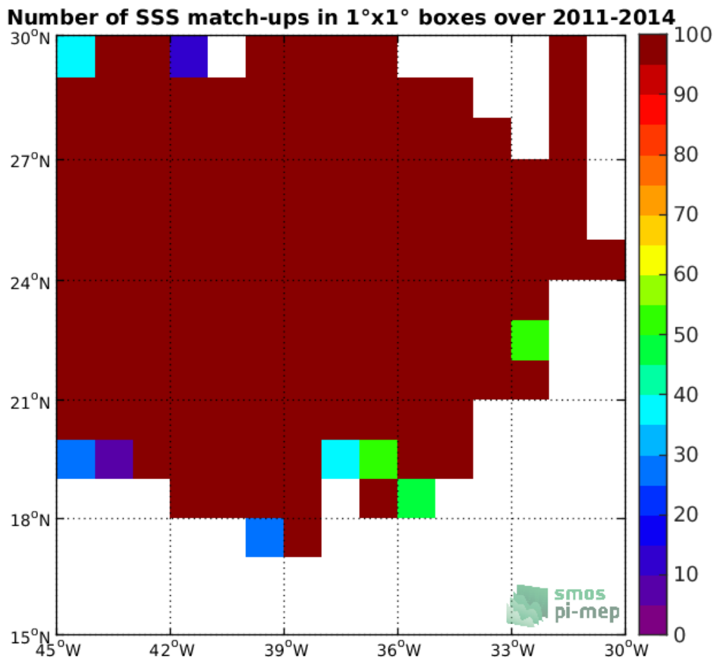
Figure 3: Number of SSS match-ups between Surface drifters SSS and the SMOS-L3-CATDS-CPDC-V317-MONTHLY-25KM SSS product for the SPURS 1 Pi-MEP region over 1°x1° boxes and for the full satellite product period.
