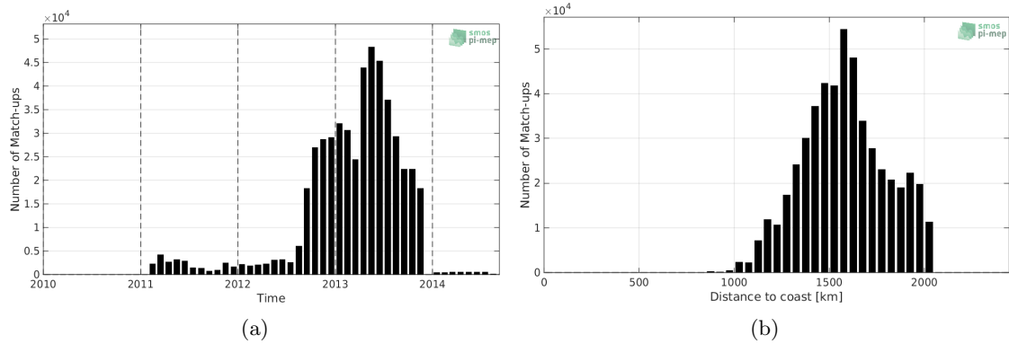
Figure 1: Number of match-ups between Surface drifters and SMOS-L3-CATDS-CPDC-V317-MONTHLY-25KM SSS as a function of time (a) and as function of the distance to coast (b) over the SPURS 1 Pi-MEP region and for the full satellite product period.
