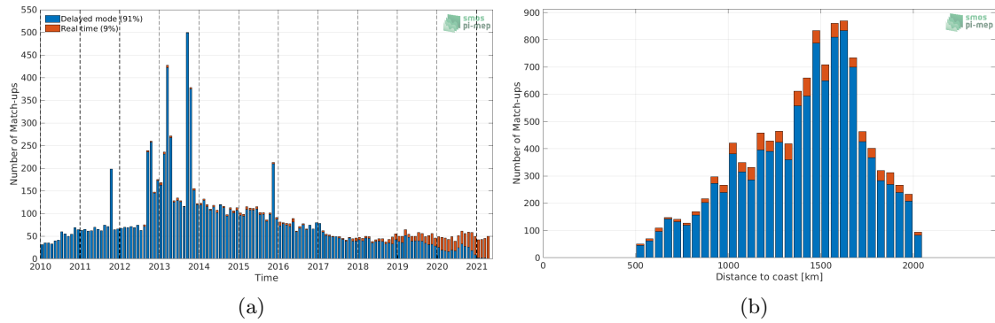
Figure 1: Number of match-ups between Argo and SMOS SSS L3 v317 - Monthly - 25 km (CATDS-CPDC) SSS as a function of time (a) and as function of the distance to coast (b) over the SPURS 1 Pi-MEP region and for the full satellite product period.
