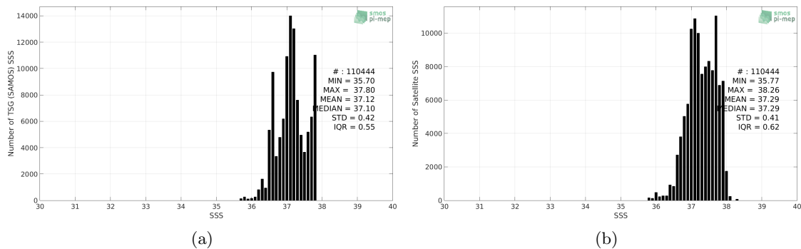
Figure 2: Histograms of SSS from TSG (SAMOS) (a) and SMOS SSS L3 v317 - 10 Days - 25 km (CATDS-CPDC) (b) considering all match-up pairs per bins of 0.1 over the SPURS 1 Pi-MEP region and for the full satellite product period.
