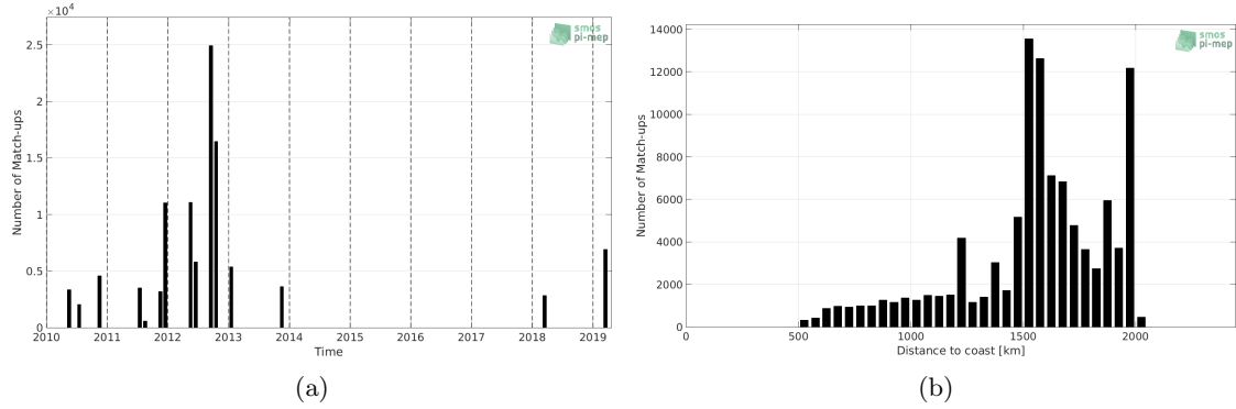
Figure 1: Number of match-ups between TSG-SAMOS and SMOS L3 v317 - 10 Days - 25 km (CATDS-CPDC) SSS as a function of time (a) and as function of the distance to coast (b) over the SPURS 1 Pi-MEP region and for the full satellite product period.
