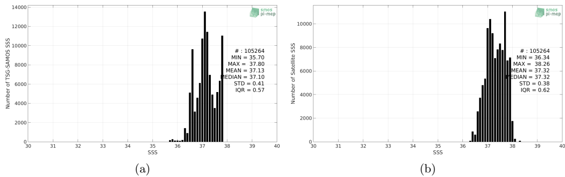
Figure 2: Histograms of SSS from TSG-SAMOS (a) and SMOS L3 v317 - 10 Days - 25 km (CATDS-CPDC) (b) considering all match-up pairs per bins of 0.1 over the SPURS 1 Pi-MEP region and for the full satellite product period.
