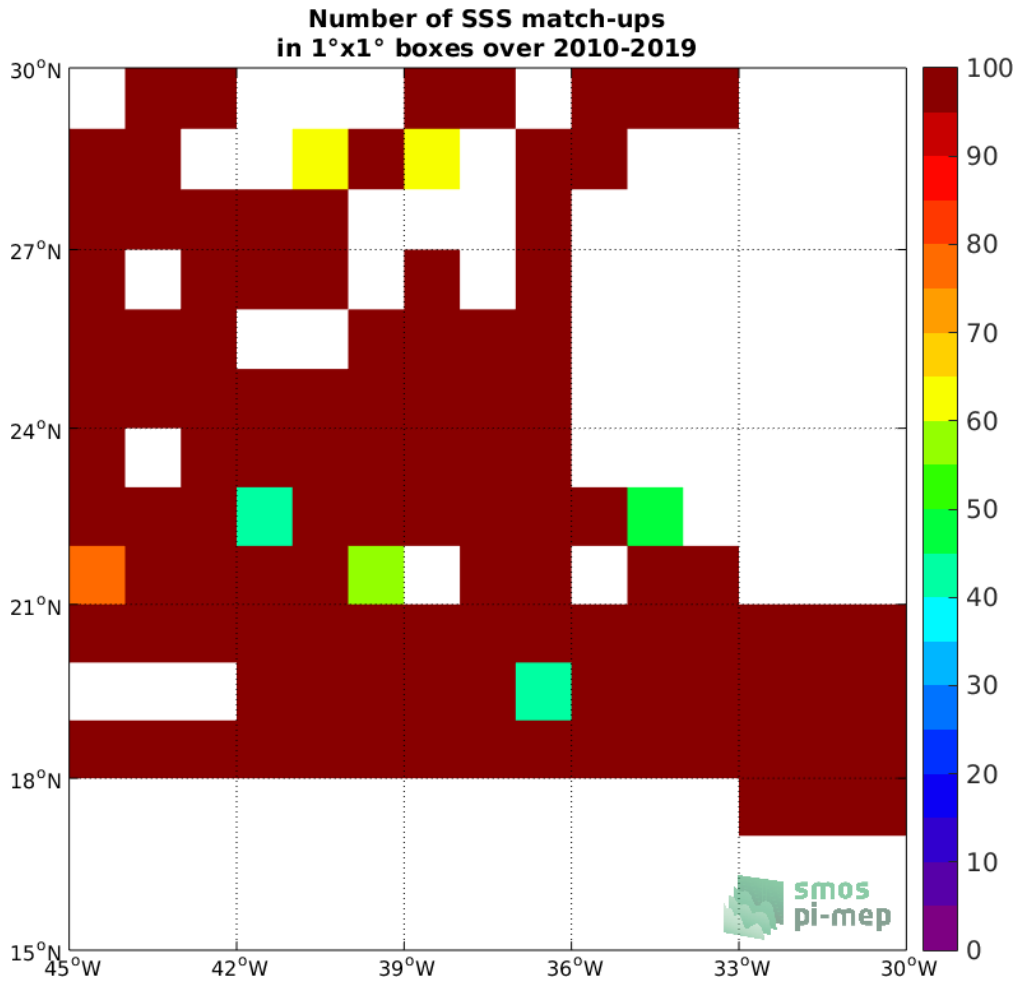
Figure 4: Number of SSS match-ups between TSG-SAMOS SSS and the SMOS L3 v317 - 10 Days - 25 km (CATDS-CPDC) SSS product for the SPURS 1 Pi-MEP region over 1°x1° boxes and for the full satellite product period.
