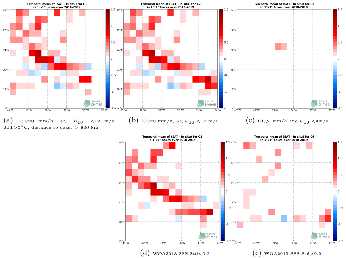
Figure 12: Temporal mean gridded over spatial boxes of size 1^\circ \times 1^\circ of \Delta\text{SSS} (SMOS-L3-CATDS-CPDC-V317-10DAYS-25KM - TSG-SAMOS) for 5 different subdatasets corresponding to:RR=0 mm/h, 3 < U_{10} < 12 m/s, SST >5^\circ\text{C} , distance to coast > 800 km (a), RR=0 mm/h, 3 < U_{10} < 12 m/s (b), RR >1 mm/h and U_{10} < 4 m/s (c), WOA2013 SSS Std <0.2 (d), WOA2013 SSS Std >0.2 (e).
