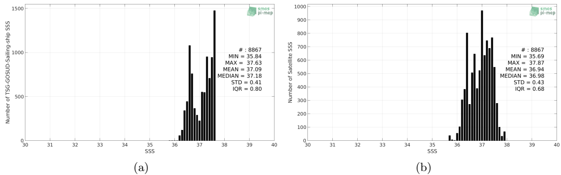
Figure 2: Histograms of SSS from TSG-GOSUD-Sailing-ship (a) and SMOS L3 v317 - 10 Days - 25 km (CATDS-CPDC) (b) considering all match-up pairs per bins of 0.1 over the SPURS 1 Pi-MEP region and for the full satellite product period.
