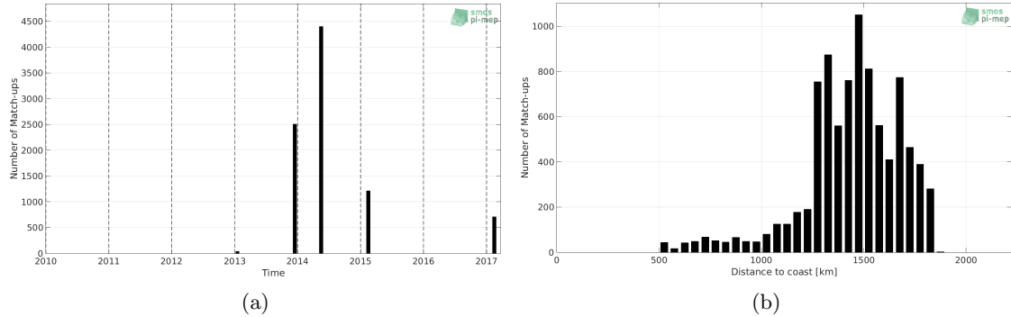
Figure 1: Number of match-ups between TSG-GOSUD-Sailing-ship and SMOS L3 v317 - 10 Days - 25 km (CATDS-CPDC) SSS as a function of time (a) and as function of the distance to coast (b) over the SPURS 1 Pi-MEP region and for the full satellite product period.
