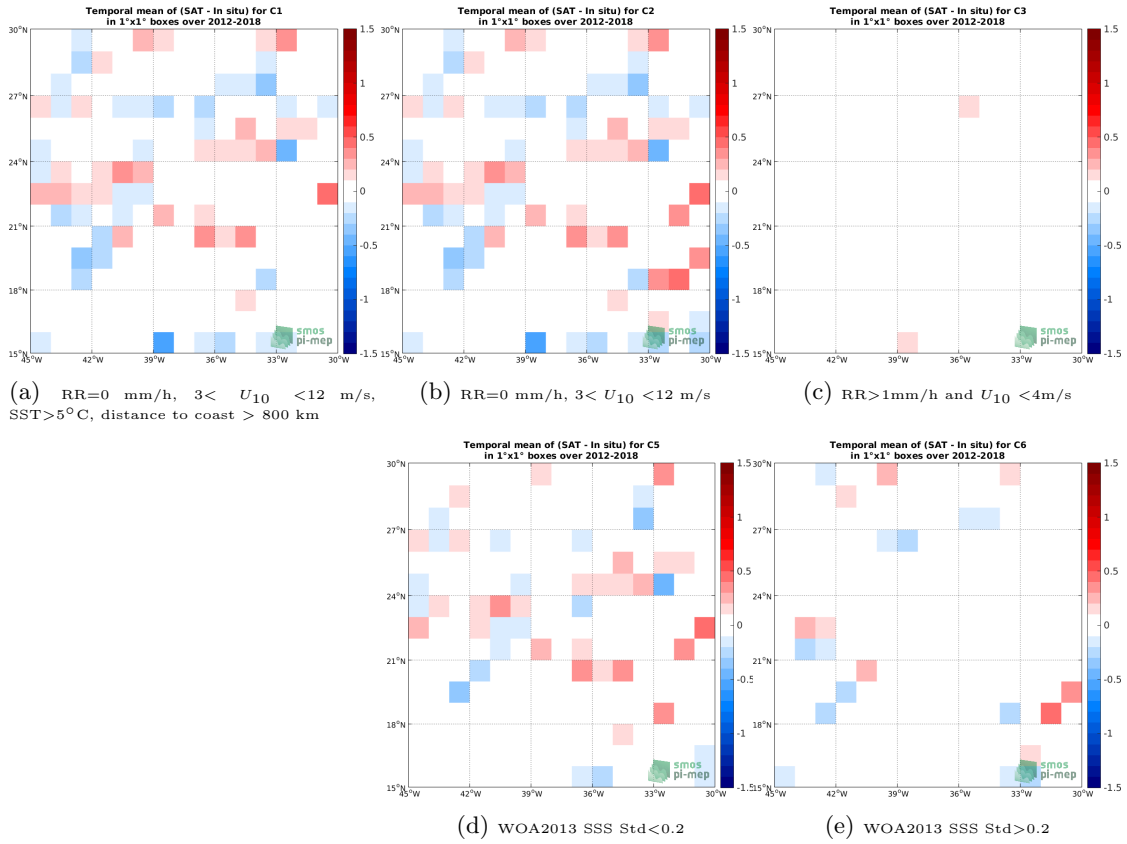
Figure 12: Temporal mean gridded over spatial boxes of size 1°x1° of \Delta SSS (SMOS SSS L3 v317 - 10 Days - 25 km (CATDS-CPDC) - TSG (GOSUD-Research-vessel)) for 5 different subdatasets corresponding to: RR=0 mm/h, 3 < U_{10} < 12 m/s, SST>5°C, distance to coast > 800 km (a), RR=0 mm/h, 3 < U_{10} < 12 m/s (b), RR>1mm/h and U_{10} < 4 m/s (c), WOA2013 SSS Std<0.2 (d), WOA2013 SSS Std>0.2 (e).
