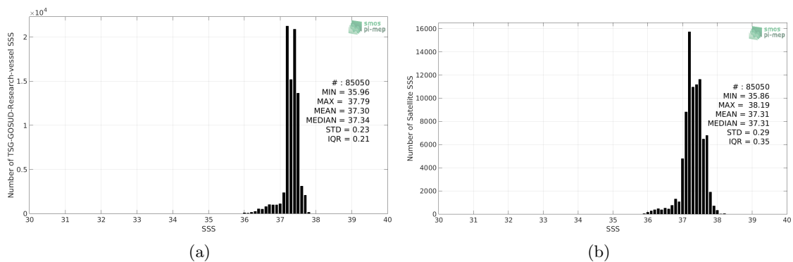
Figure 2: Histograms of SSS from TSG-GOSUD-Research-vessel (a) and SMOS L3 v317 - 10 Days - 25 km (CATDS-CPDC) (b) considering all match-up pairs per bins of 0.1 over the SPURS 1 Pi-MEP region and for the full satellite product period.
