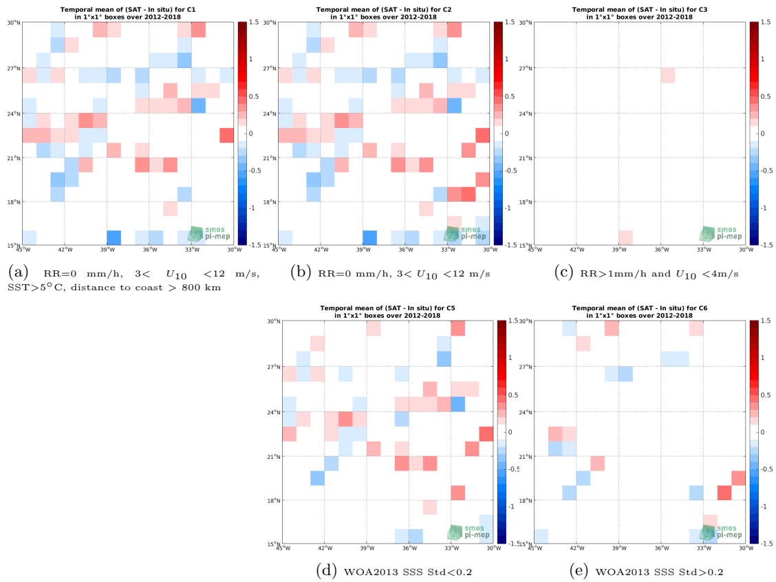
Figure 12: Temporal mean gridded over spatial boxes of size 1^\circ \times 1^\circ of \Delta SS (SMOS L3 v317 - 10 Days - 25 km (CATDS-CPDC) - TSG-GOSUD-Research-vessel) for 5 different subdatasets corresponding to: RR=0 mm/h, 3 < U_{10} < 12 m/s, SST>5°C, distance to coast > 800 km (a), RR=0 mm/h, 3 < U_{10} < 12 m/s (b), RR>1mm/h and U_{10} < 4 m/s (c), WOA2013 SSS Std<0.2 (d), WOA2013 SSS Std>0.2 (e).
