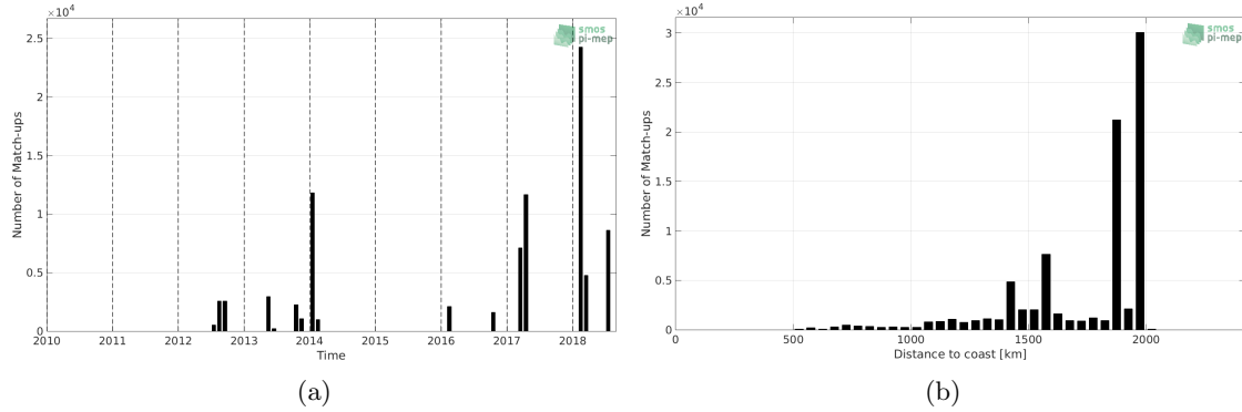
Figure 1: Number of match-ups between TSG-GOSUD-Research-vessel and SMOS L3 v317 - 10 Days - 25 km (CATDS-CPDC) SSS as a function of time (a) and as function of the distance to coast (b) over the SPURS 1 Pi-MEP region and for the full satellite product period.
