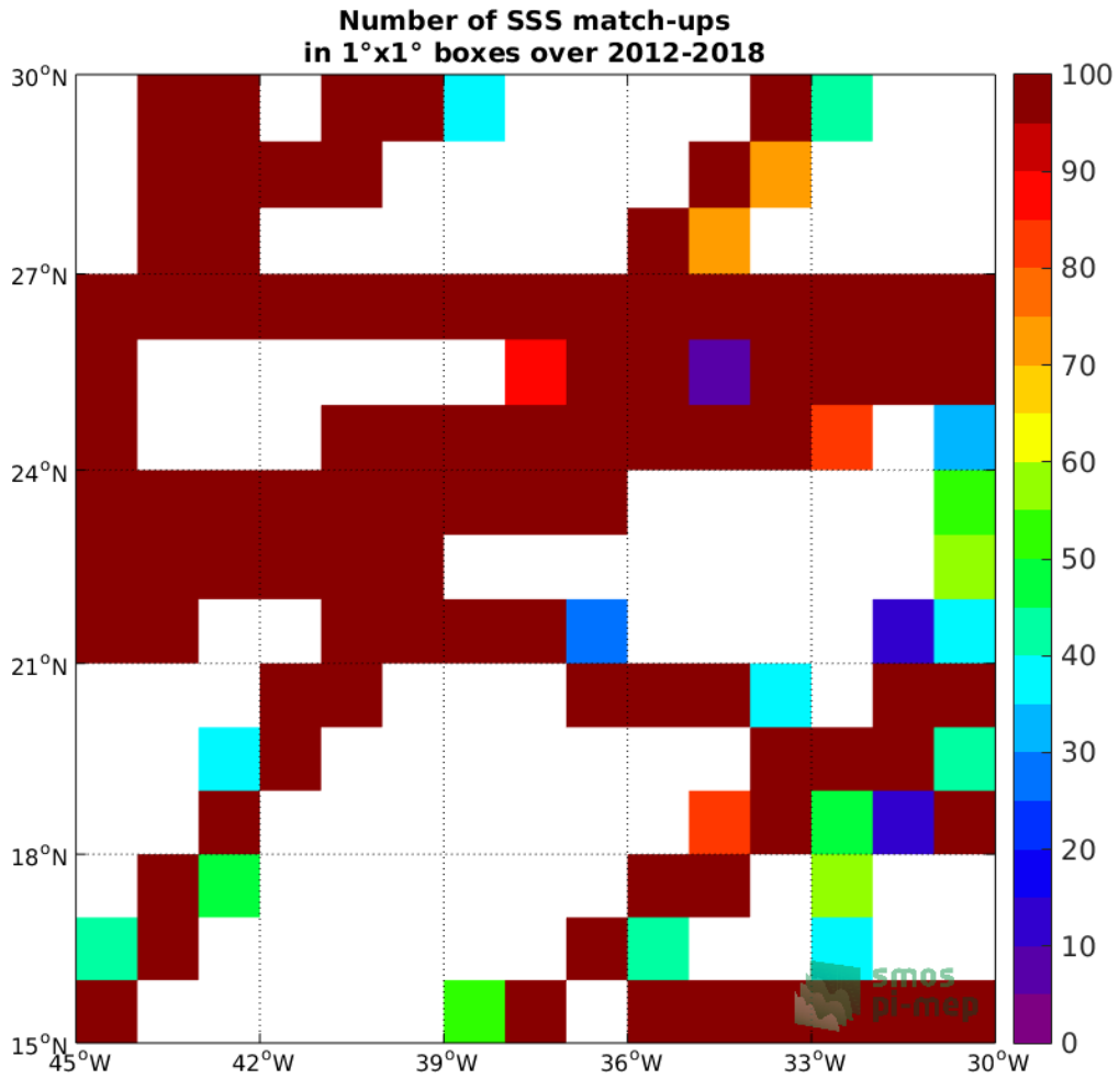
Figure 4: Number of SSS match-ups between TSG-GOSUD-Research-vessel SSS and the SMOS L3 v317 - 10 Days - 25 km (CATDS-CPDC) SSS product for the SPURS 1 Pi-MEP region over 1°x1° boxes and for the full satellite product period.
