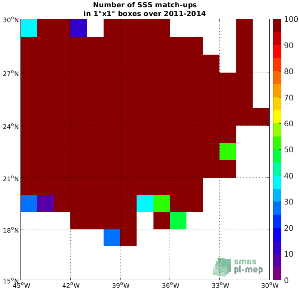
Figure 3: Number of SSS match-ups between Surface drifters SSS and the SMOS SSS L3 v317 - 10 Days - 25 km (CATDS-CPDC) SSS product for the SPURS 1 Pi-MEP region over 1^\circ \times 1^\circ boxes and for the full satellite product period.
