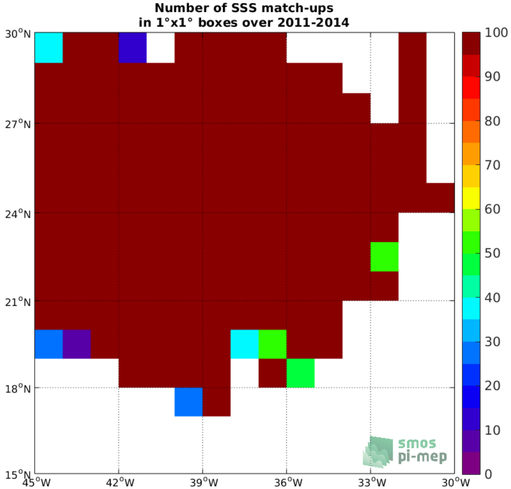
Figure 3: Number of SSS match-ups between Surface drifters SSS and the SMOS SSS L3 v317 - 10 Days - 25 km (CATDS-CPDC) SSS product for the SPURS 1 Pi-MEP region over 1°x1° boxes and for the full satellite product period.
