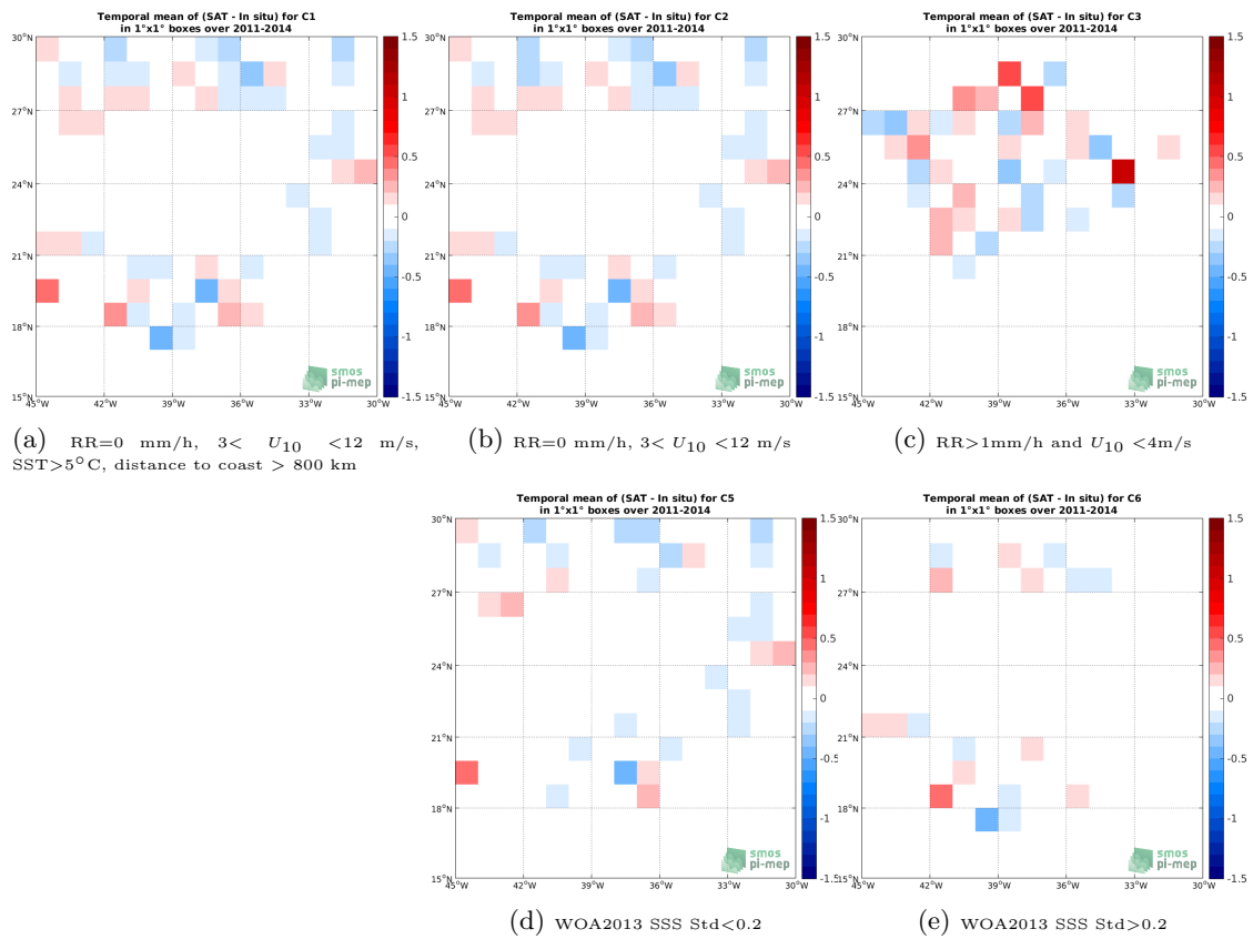
Figure 11: Temporal mean gridded over spatial boxes of size 1^\circ \times 1^\circ of \Delta\text{SSS} (SMOS SSS L3 v317 - 10 Days - 25 km (CATDS-CPDC) - Surface drifters) for 5 different subdatasets corresponding to:RR=0 mm/h, 3 < U_{10} < 12 m/s, SST >5^\circ\text{C} , distance to coast > 800 km (a), RR=0 mm/h, 3 < U_{10} < 12 m/s (b), RR >1 mm/h and U_{10} < 4 m/s (c), WOA2013 SSS Std <0.2 (d), WOA2013 SSS Std >0.2 (e).
