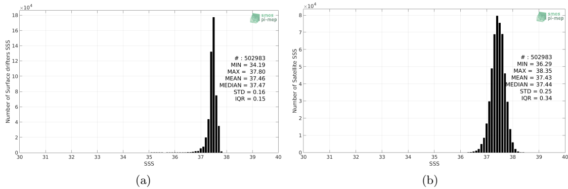
Figure 2: Histograms of SSS from Surface drifters (a) and SMOS SSS L3 v317 - 10 Days - 25 km (CATDS-CPDC) (b) considering all match-up pairs per bins of 0.1 over the SPURS 1 Pi-MEP region and for the full satellite product period.
