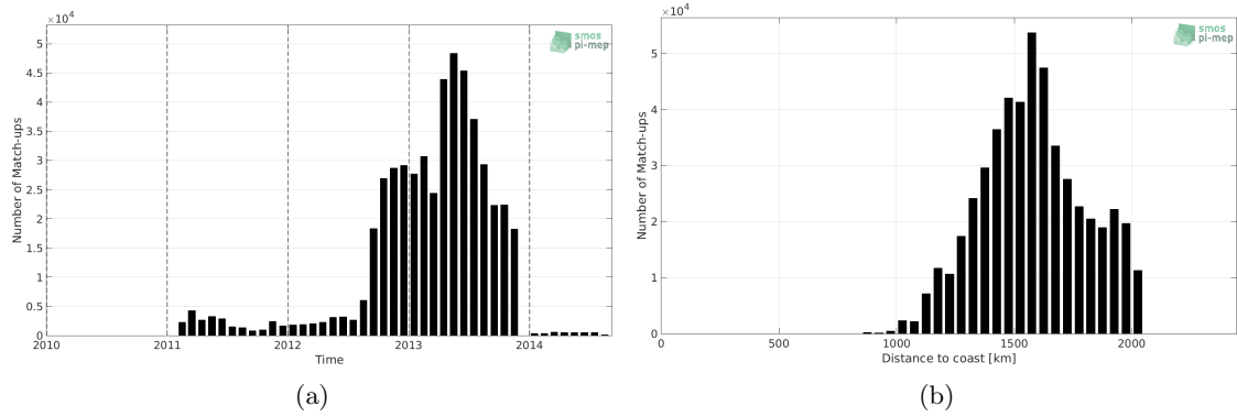
Figure 1: Number of match-ups between Surface drifters and SMOS SSS L3 v317 - 10 Days - 25 km (CATDS-CPDC) SSS as a function of time (a) and as function of the distance to coast (b) over the SPURS 1 Pi-MEP region and for the full satellite product period.
