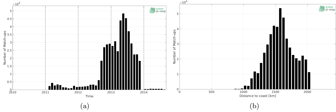
Figure 1: Number of match-ups between Surface drifters and SMOS L3 v317 - 10 Days - 25 km (CATDS-CPDC) SSS as a function of time (a) and as function of the distance to coast (b) over the SPURS 1 Pi-MEP region and for the full satellite product period.
