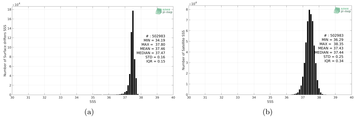
Figure 2: Histograms of SSS from Surface drifters (a) and SMOS L3 v317 - 10 Days - 25 km (CATDS-CPDC) (b) considering all match-up pairs per bins of 0.1 over the SPURS 1 Pi-MEP region and for the full satellite product period.
