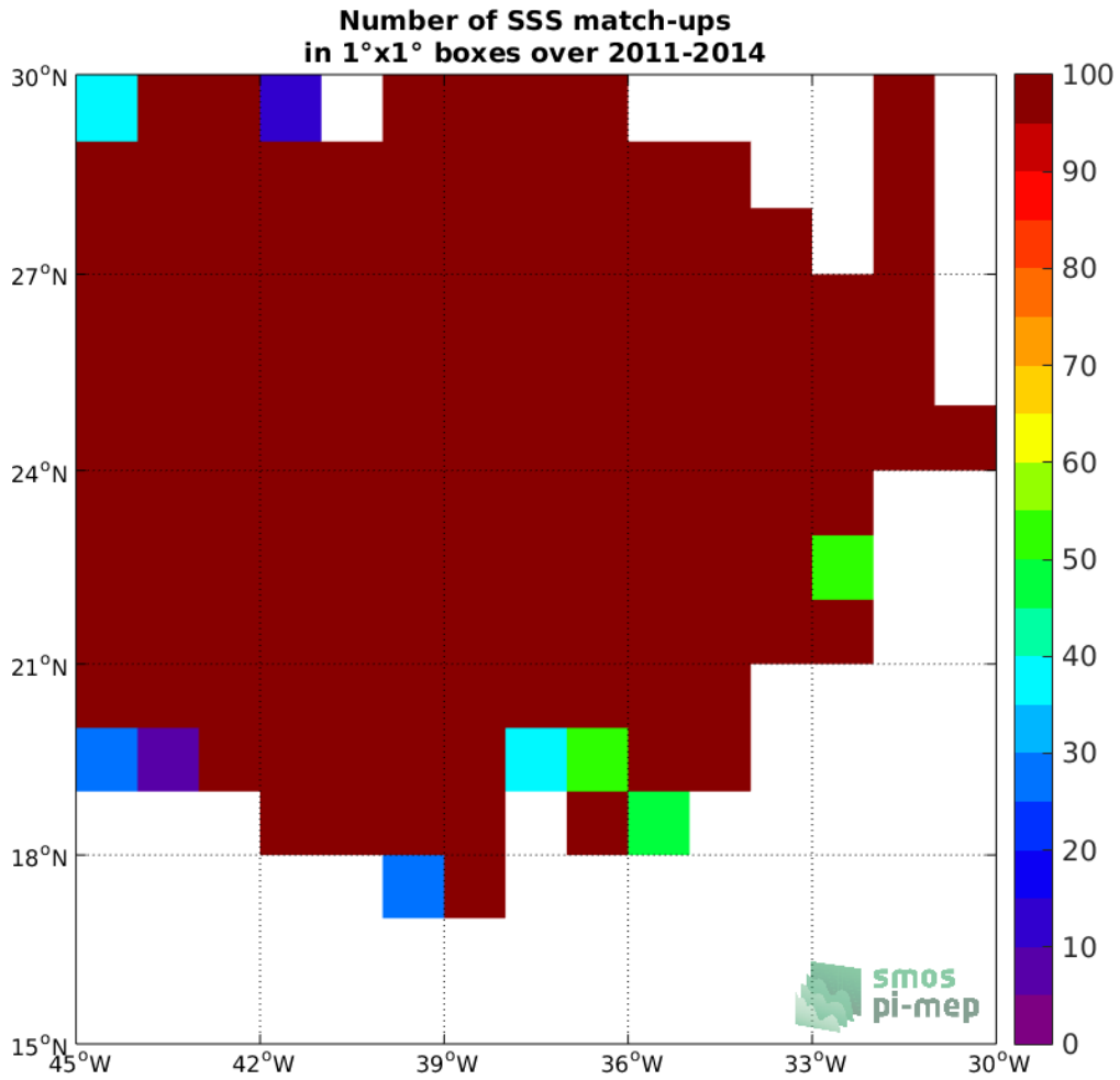
Figure 3: Number of SSS match-ups between Surface drifters SSS and the SMOS L3 v317 - 10 Days - 25 km (CATDS-CPDC) SSS product for the SPURS 1 Pi-MEP region over 1°x1° boxes and for the full satellite product period.
