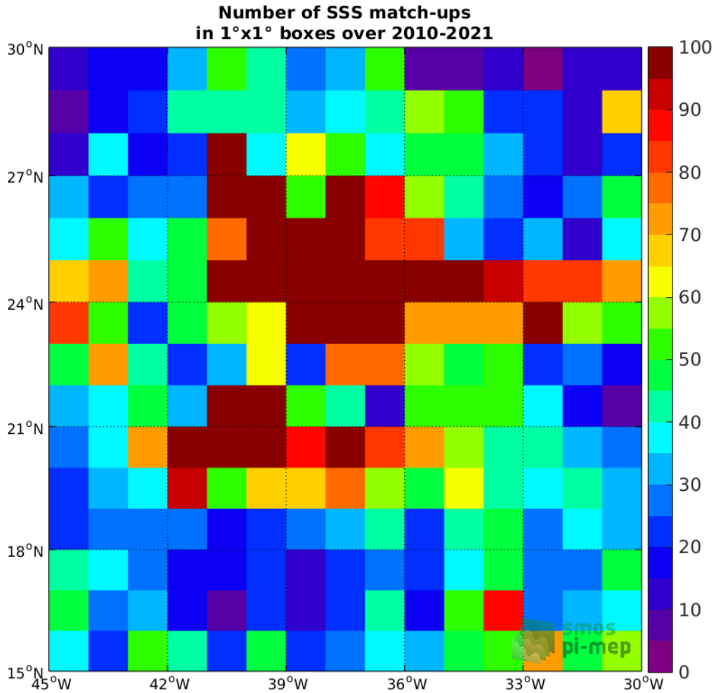
Figure 4: Number of SSS match-ups between Argo SSS and the SMOS SSS L3 v317 - 10 Days - 25 km (CATDS-CPDC) SSS product for the SPURS 1 Pi-MEP region over 1^\circ \times 1^\circ boxes and for the full satellite product period.
