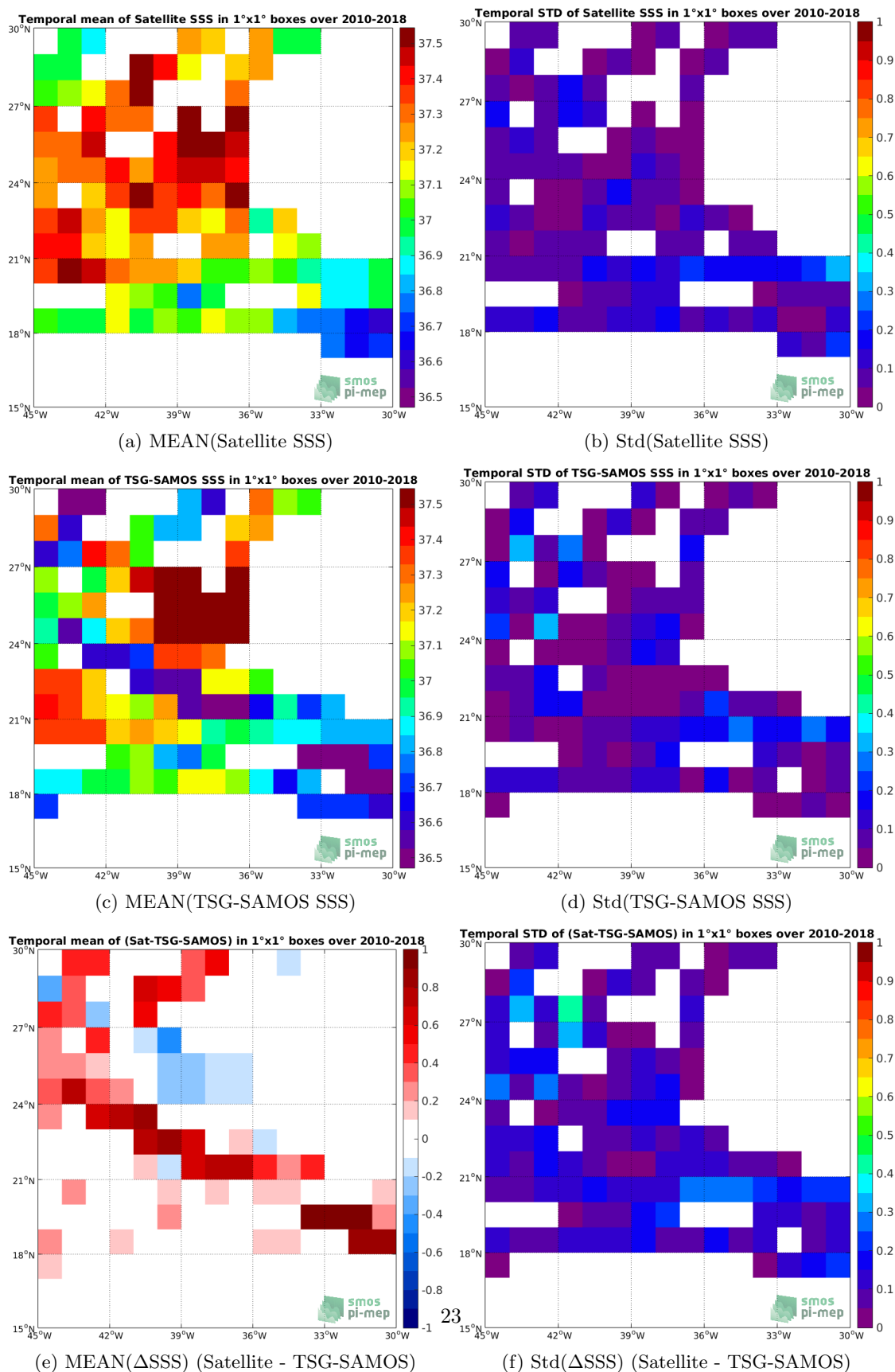
Figure 6: Temporal mean (left) and Std (right) of SSS from SMOS-L3-CATDS-CPDC-V3-MONTHLY-25KM (top), TSG-SAMOS (middle), and of \Delta SSS (Satellite - TSG-SAMOS). Only match-up pairs are used to generate these maps.
