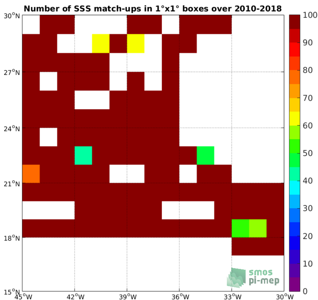
Figure 4: Number of SSS match-ups between TSG-SAMOS SSS and the SMOS-L3-CATDS-CPDC-V3-MONTHLY-25KM SSS product for the SPURS 1 Pi-MEP region over 1°x1° boxes and for the full satellite product period.
