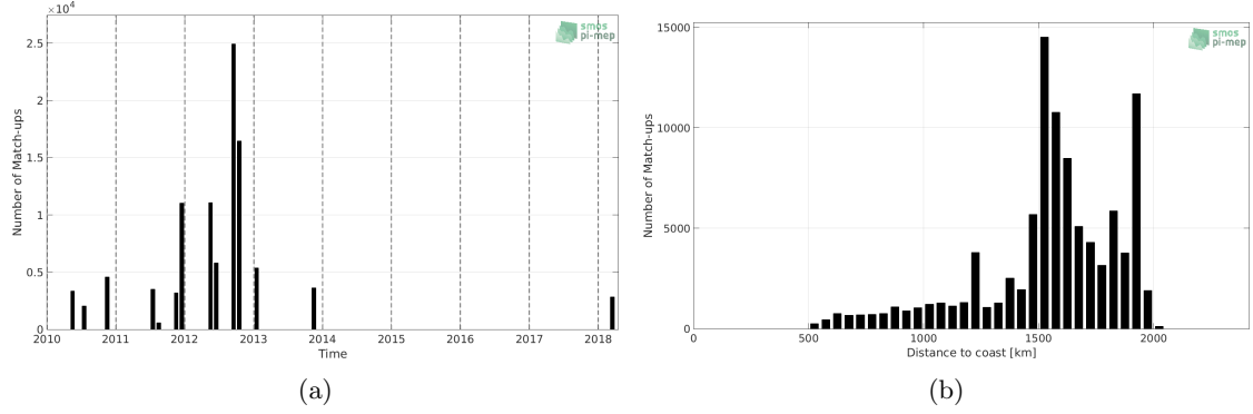
Figure 1: Number of match-ups between TSG-SAMOS and SMOS-L3-CATDS-CPDC-V3-MONTHLY-25KM SSS as a function of time (a) and as function of the distance to coast (b) over the SPURS 1 Pi-MEP region and for the full satellite product period.
