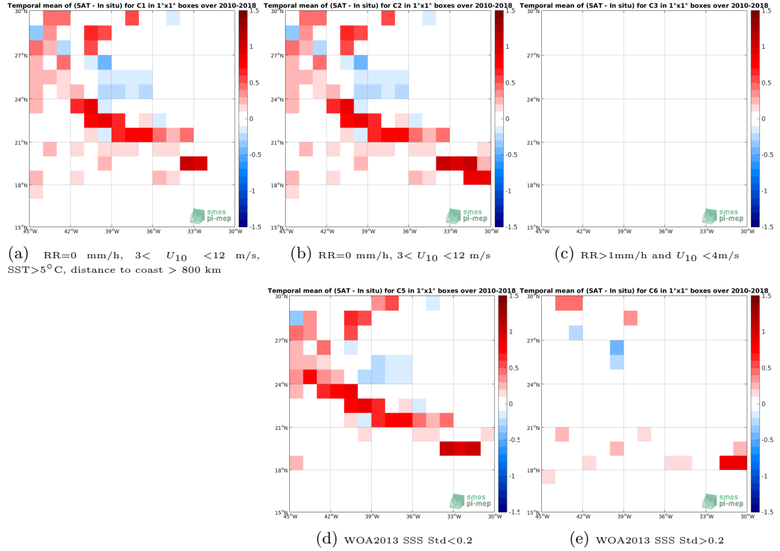
Figure 12: Temporal mean gridded over spatial boxes of size 1^\circ \times 1^\circ of \Delta SSS (SMOS-L3-CATDS-CPDC-V3-MONTHLY-25KM - TSG-SAMOS) for 5 different subdatasets corresponding to: RR=0 mm/h, 3 < U_{10} < 12 m/s, SST > 5^\circ\text{C} , distance to coast > 800 km (a), RR=0 mm/h, 3 < U_{10} < 12 m/s (b), RR > 1 mm/h and U_{10} < 4 m/s (c), WOA2013 SSS Std < 0.2 (d), WOA2013 SSS Std > 0.2 (e).
