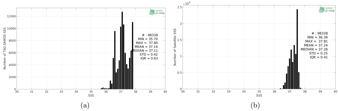
Figure 2: Histograms of SSS from TSG-SAMOS (a) and SMOS-L3-CATDS-CPDC-V3-MONTHLY-25KM (b) considering all match-up pairs per bins of 0.1 over the SPURS 1 Pi-MEP region and for the full satellite product period.
