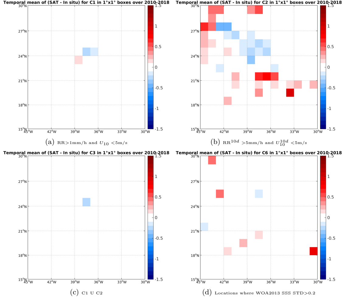
Figure 12: Temporal mean gridded over spatial boxes of size 1^\circ \times 1^\circ of \Delta SSS (SMOS-L3-CATDS-CPDC-V3-MONTHLY-25KM - TSG-SAMOS) for 4 different subdatasets corresponding to: RR > 1\text{mm/h} and U_{10} < 5\text{m/s} (a), RR^{10d} > 5\text{mm/h} and U_{10}^{10d} < 5\text{m/s} (b), C1 U C2 (c), Locations where WOA2013 SSS STD > 0.2 (d).
