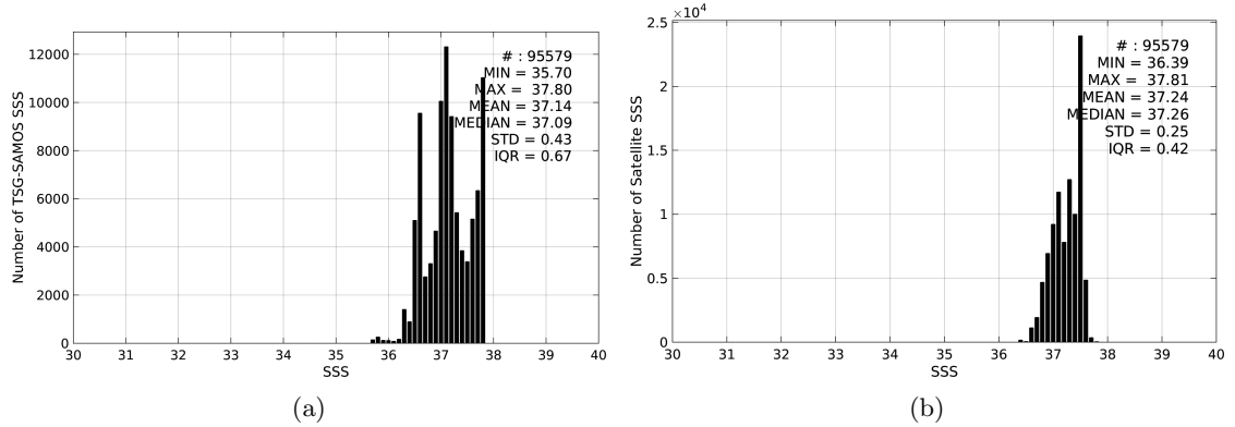
Figure 2: Histograms of SSS from TSG-SAMOS (a) and SMOS-L3-CATDS-CPDC-V3-MONTHLY-25KM (b) considering all match-up pairs per bins of 0.1 over the SPURS 1 Pi-MEP region and for the full satellite product period.
