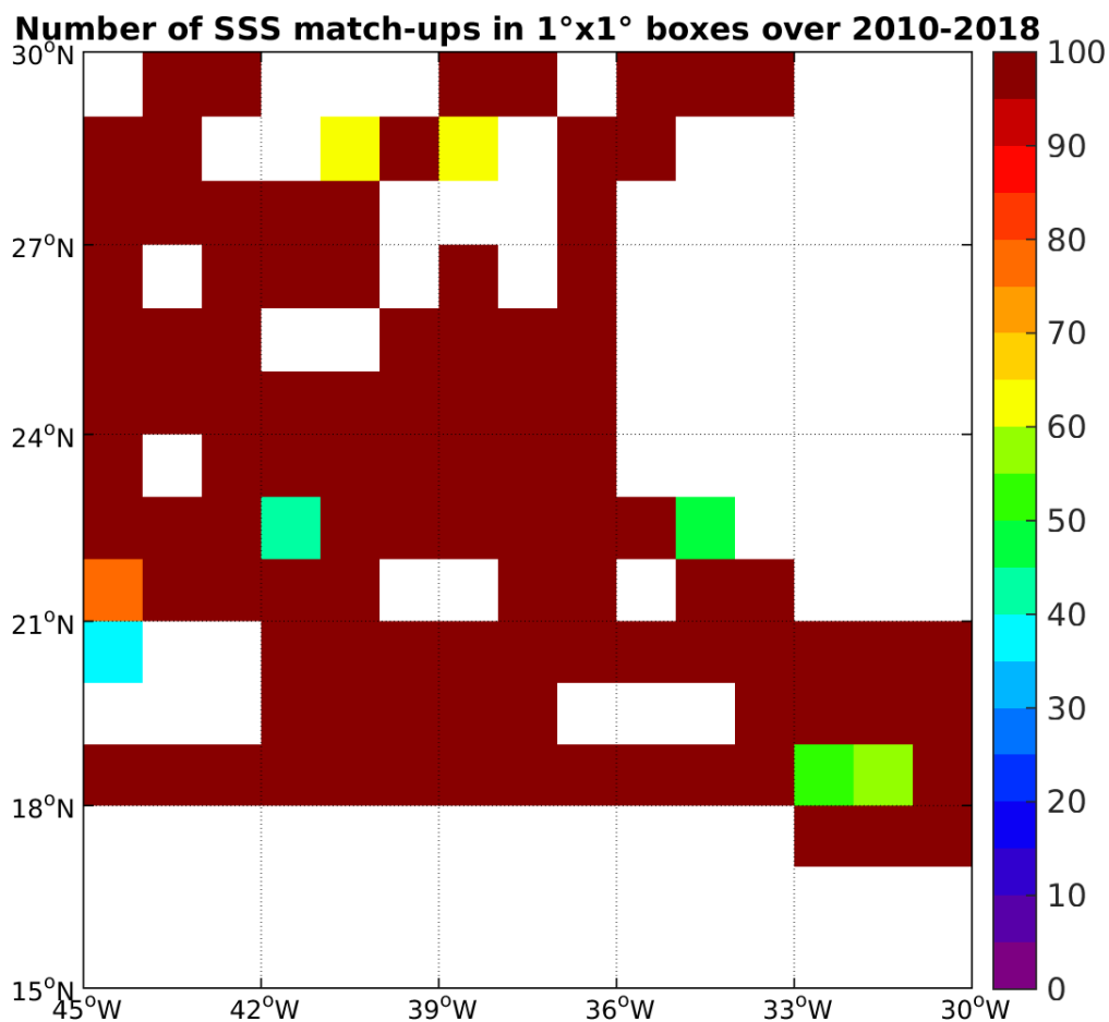
Figure 4: Number of SSS match-ups between TSG-SAMOS SSS and the SMOS-L3-CATDS-CPDC-V3-MONTHLY-25KM SSS product for the SPURS 1 Pi-MEP region over 1°x1° boxes and for the full satellite product period.
