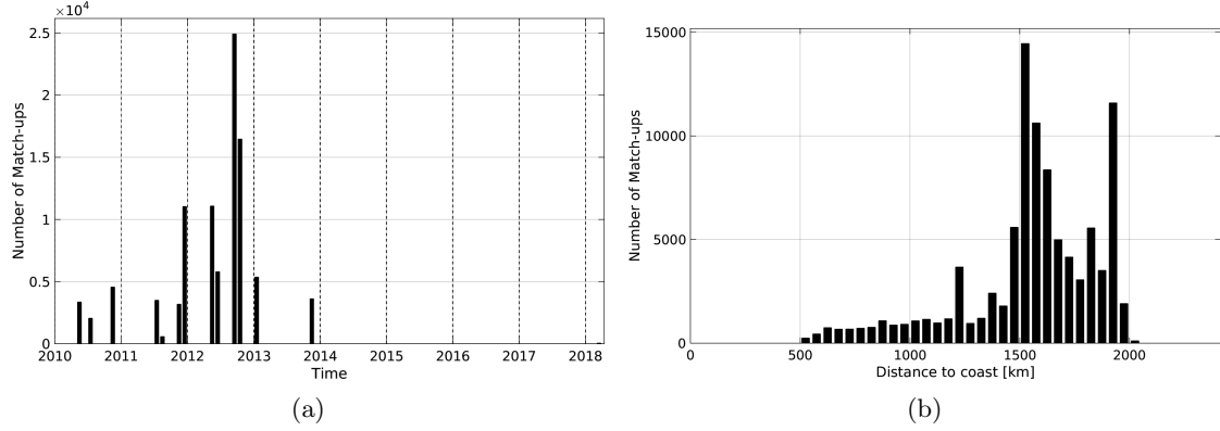
Figure 1: Number of match-ups between TSG-SAMOS and SMOS-L3-CATDS-CPDC-V3-MONTHLY-25KM SSS as a function of time (a) and as function of the distance to coast (b) over the SPURS 1 Pi-MEP region and for the full satellite product period.
