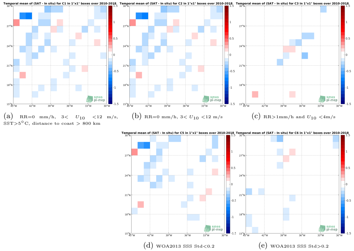
Figure 12: Temporal mean gridded over spatial boxes of size 1^\circ \times 1^\circ of \Delta SSS (SMOS-L3-CATDS-CPDC-V3-MONTHLY-25KM - TSG-LEGOS-DM) for 5 different subdatasets corresponding to: RR=0 mm/h, 3 < U_{10} < 12 m/s, SST > 5^\circ C , distance to coast > 800 km (a), RR=0 mm/h, 3 < U_{10} < 12 m/s (b), RR > 1 mm/h and U_{10} < 4 m/s (c), WOA2013 SSS Std < 0.2 (d), WOA2013 SSS Std > 0.2 (e).
