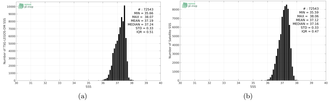
Figure 2: Histograms of SSS from TSG-LEGOS-DM (a) and SMOS-L3-CATDS-CPDC-V3-MONTHLY-25KM (b) considering all match-up pairs per bins of 0.1 over the SPURS 1 Pi-MEP region and for the full satellite product period.
