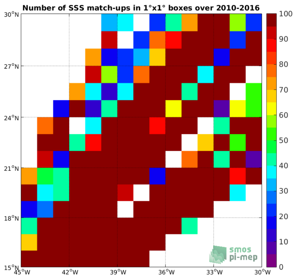
Figure 4: Number of SSS match-ups between TSG-LEGOS-DM SSS and the SMOS-L3-CATDS-CPDC-V3-MONTHLY-25KM SSS product for the SPURS 1 Pi-MEP region over 1°x1° boxes and for the full satellite product period.
