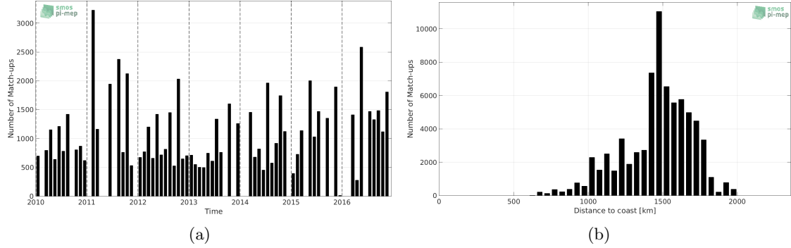
Figure 1: Number of match-ups between TSG-LEGOS-DM and SMOS-L3-CATDS-CPDC-V3-MONTHLY-25KM SSS as a function of time (a) and as function of the distance to coast (b) over the SPURS 1 Pi-MEP region and for the full satellite product period.
