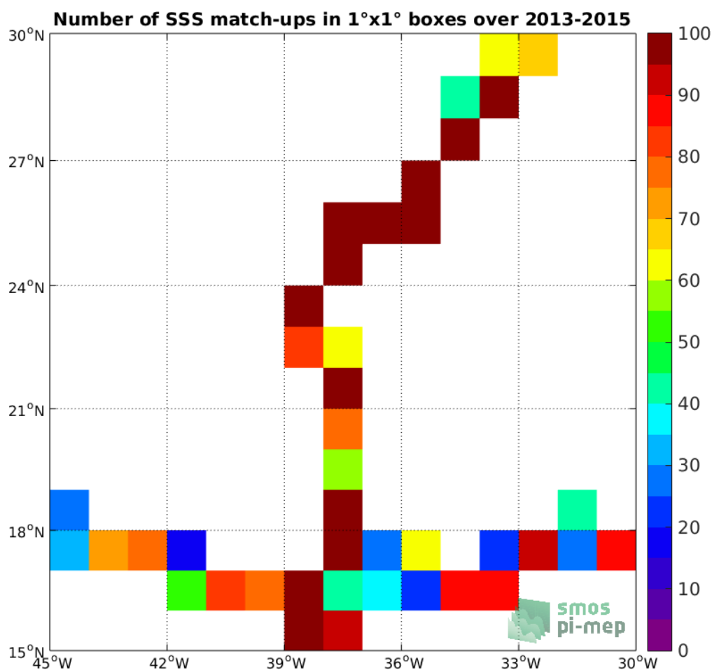
Figure 4: Number of SSS match-ups between TSG-GOSUD-Sailing-ship SSS and the SMOS-L3-CATDS-CPDC-V3-MONTHLY-25KM SSS product for the SPURS 1 Pi-MEP region over 1°x1° boxes and for the full satellite product period.
