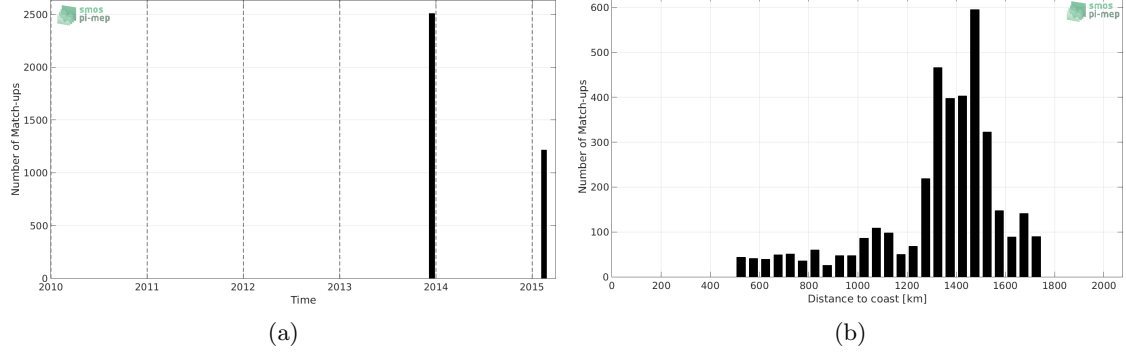
Figure 1: Number of match-ups between TSG-GOSUD-Sailing-ship and SMOS-L3-CATDS-CPDC-V3-MONTHLY-25KM SSS as a function of time (a) and as function of the distance to coast (b) over the SPURS 1 Pi-MEP region and for the full satellite product period.
