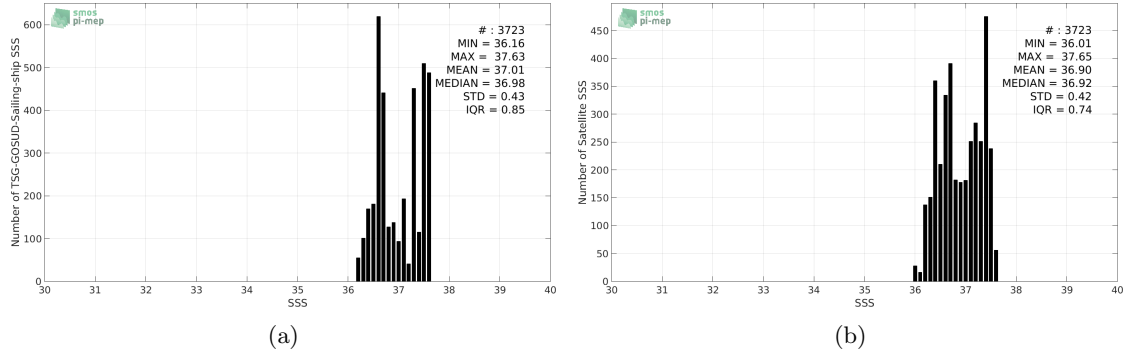
Figure 2: Histograms of SSS from TSG-GOSUD-Sailing-ship (a) and SMOS-L3-CATDS-CPDC-V3-MONTHLY-25KM (b) considering all match-up pairs per bins of 0.1 over the SPURS 1 Pi-MEP region and for the full satellite product period.
