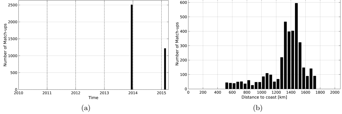
Figure 1: Number of match-ups between TSG-GOSUD-Sailing-ship and SMOS-L3-CATDS-CPDC-V3-MONTHLY-25KM SSS as a function of time (a) and as function of the distance to coast (b) over the SPURS 1 Pi-MEP region and for the full satellite product period.
