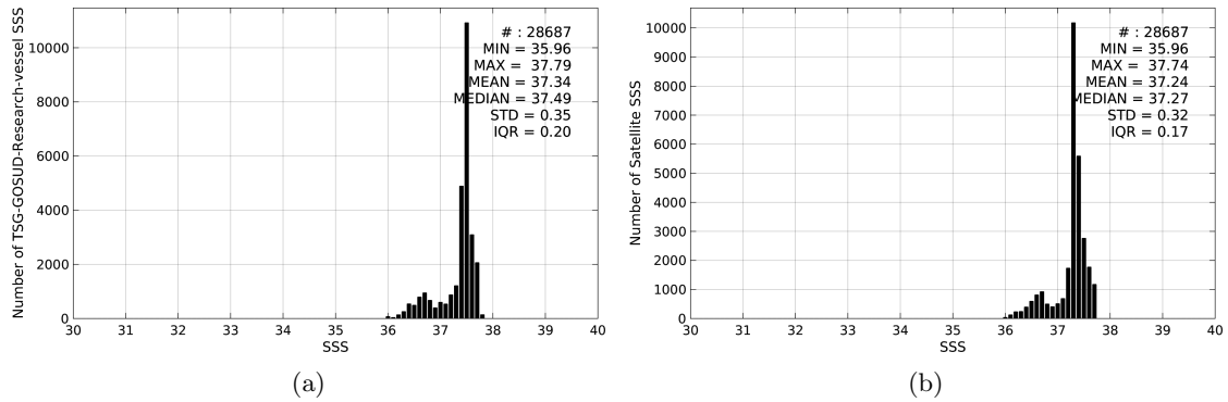
Figure 2: Histograms of SSS from TSG-GOSUD-Research-vessel (a) and SMOS-L3-CATDS-CPDC-V3-MONTHLY-25KM (b) considering all match-up pairs per bins of 0.1 over the SPURS 1 Pi-MEP region and for the full satellite product period.
