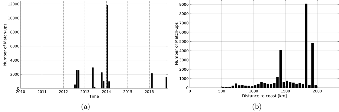
Figure 1: Number of match-ups between TSG-GOSUD-Research-vessel and SMOS-L3-CATDS-CPDC-V3-MONTHLY-25KM SSS as a function of time (a) and as function of the distance to coast (b) over the SPURS 1 Pi-MEP region and for the full satellite product period.
