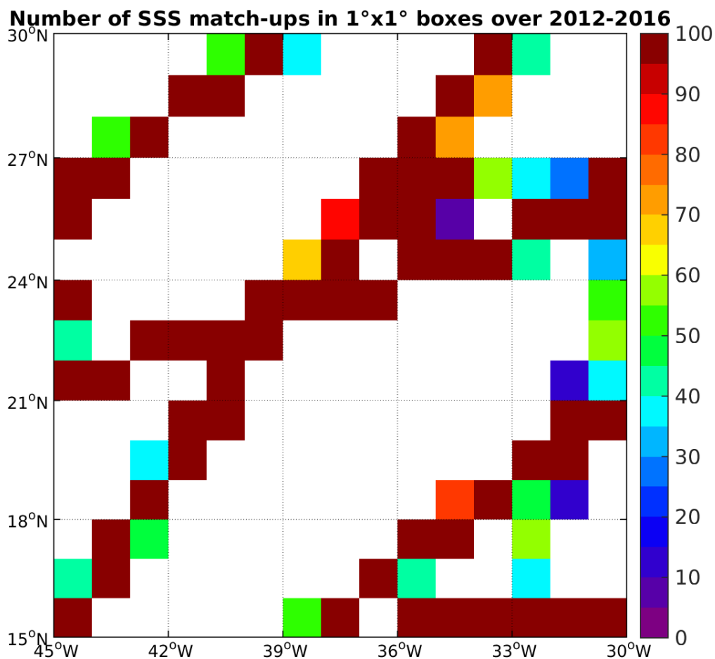
Figure 4: Number of SSS match-ups between TSG-GOSUD-Research-vessel SSS and the SMOS-L3-CATDS-CPDC-V3-MONTHLY-25KM SSS product for the SPURS 1 Pi-MEP region over 1°x1° boxes and for the full satellite product period.
