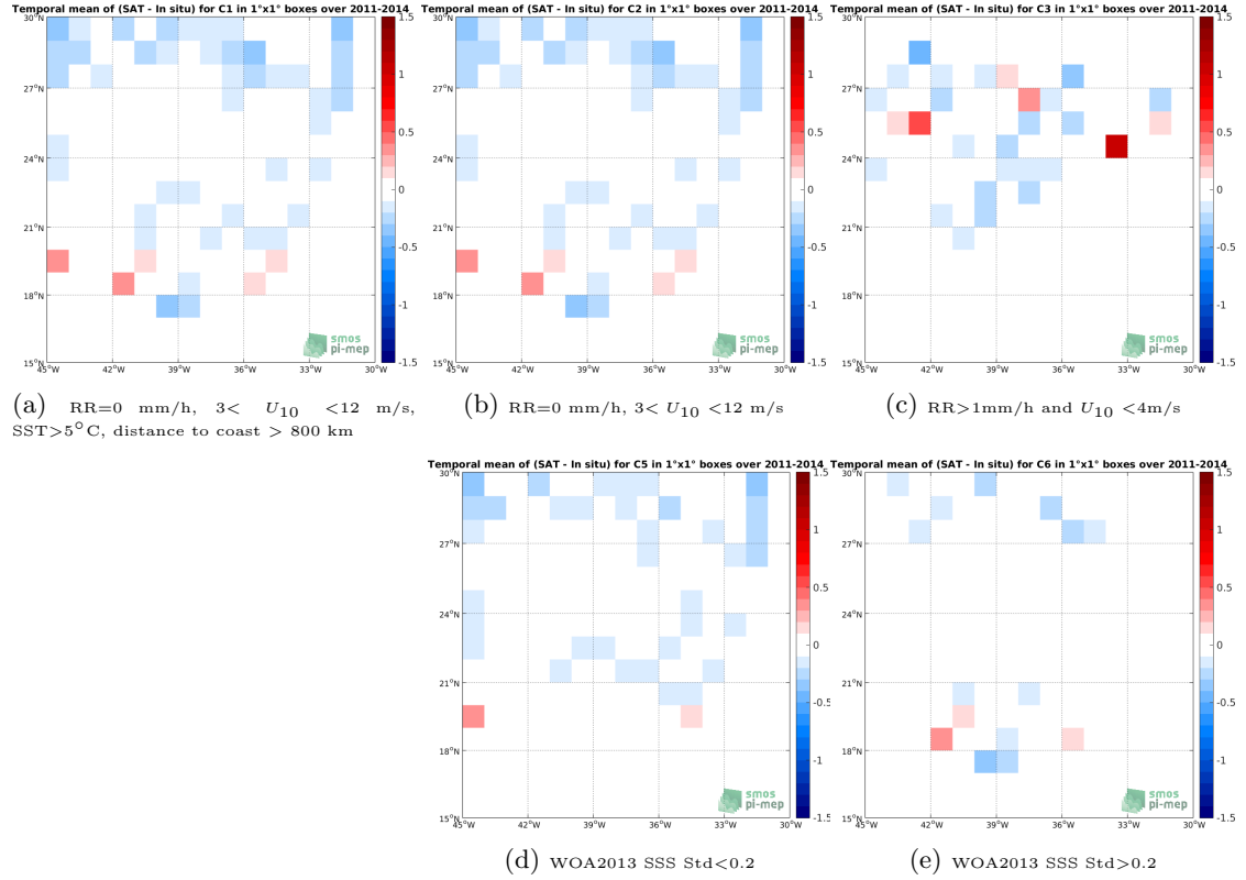
Figure 11: Temporal mean gridded over spatial boxes of size 1^\circ \times 1^\circ of \Delta SSS (SMOS-L3-CATDS-CPDC-V3-MONTHLY-25KM - Surface drifters) for 5 different subdatasets corresponding to: RR=0 mm/h, 3 < U_{10} < 12 m/s, SST > 5^\circ C , distance to coast > 800 km (a), RR=0 mm/h, 3 < U_{10} < 12 m/s (b), RR > 1 mm/h and U_{10} < 4 m/s (c), WOA2013 SSS Std < 0.2 (d), WOA2013 SSS Std > 0.2 (e).
