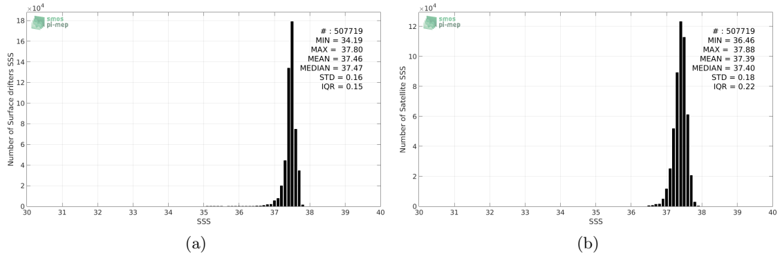
Figure 2: Histograms of SSS from Surface drifters (a) and SMOS-L3-CATDS-CPDC-V3-MONTHLY-25KM (b) considering all match-up pairs per bins of 0.1 over the SPURS 1 Pi-MEP region and for the full satellite product period.
