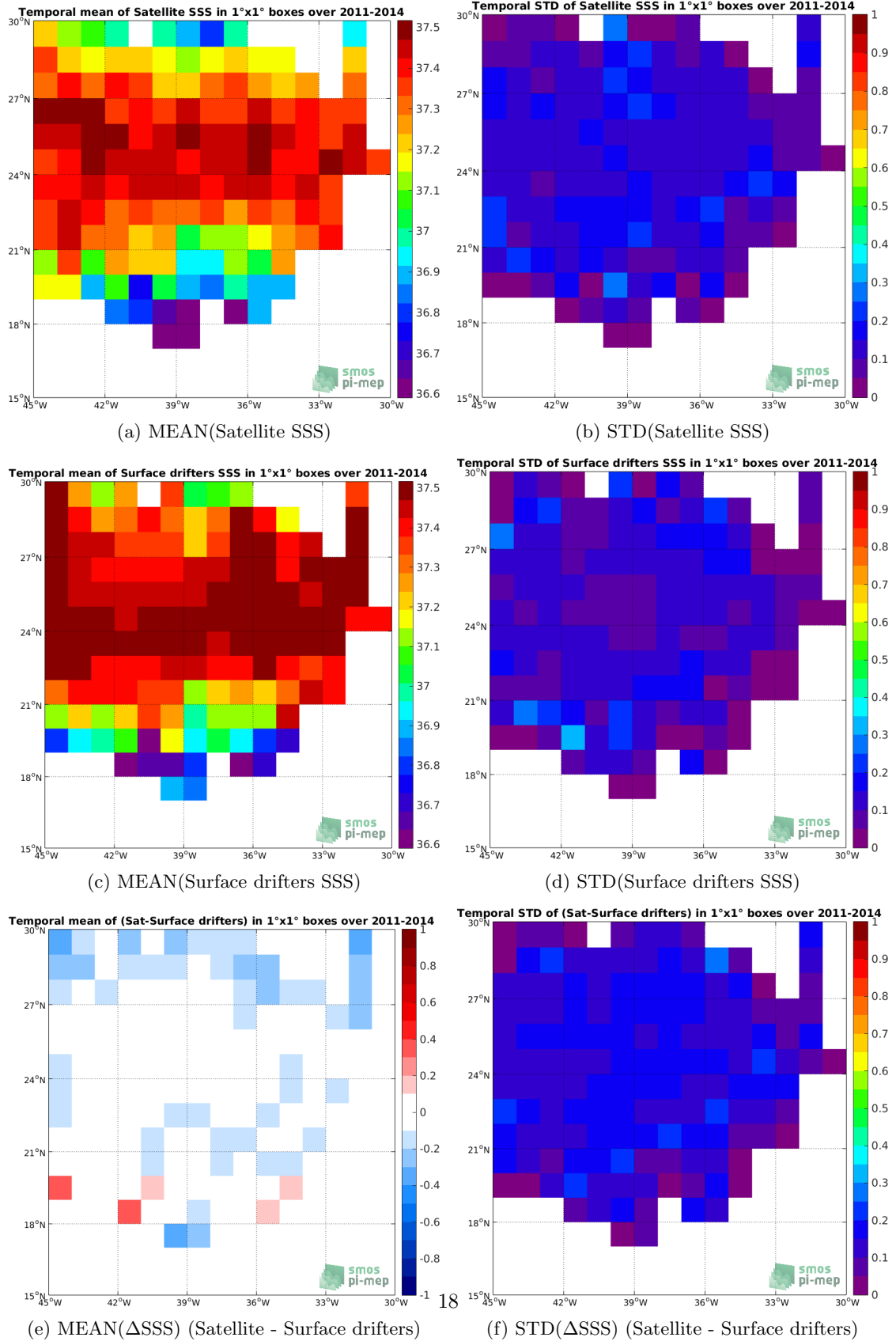
Figure 5: Temporal mean (left) and STD (right) of SSS from SMOS-L3-CATDS-CPDC-V3-MONTHLY-25KM (top), Surface drifters (middle), and of \Delta SSS (Satellite - Surface drifters). Only match-up pairs are used to generate these maps.
