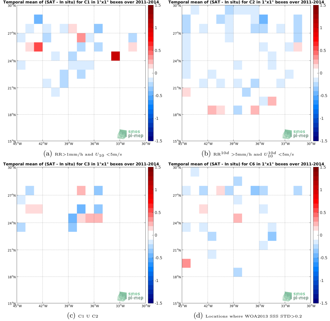
Figure 11: Temporal mean gridded over spatial boxes of size 1^\circ \times 1^\circ of \Delta SSS (SMOS-L3-CATDS-CPDC-V3-MONTHLY-25KM - Surface drifters) for 4 different subdatasets corresponding to: RR > 1\text{mm/h} and U_{10} < 5\text{m/s} (a), RR^{10d} > 5\text{mm/h} and U_{10}^{10d} < 5\text{m/s} (b), C1 U C2 (c), Locations where WOA2013 SSS STD > 0.2 (d).
