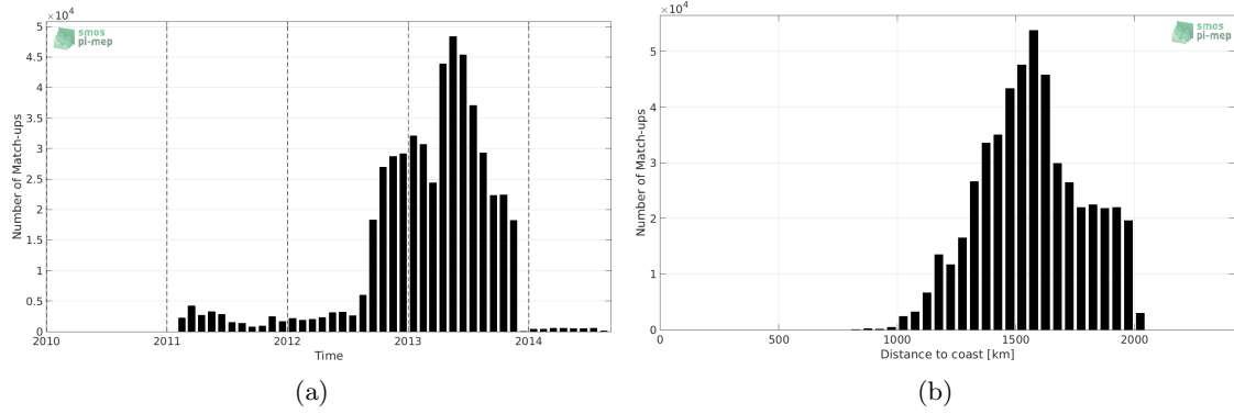
Figure 1: Number of match-ups between Surface drifters and SMOS-L3-CATDS-CPDC-V3-MONTHLY-25KM SSS as a function of time (a) and as function of the distance to coast (b) over the SPURS 1 Pi-MEP region and for the full satellite product period.
