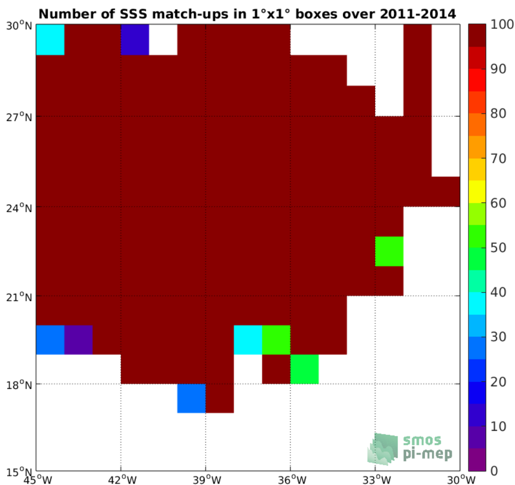
Figure 3: Number of SSS match-ups between Surface drifters SSS and the SMOS-L3-CATDS-CPDC-V3-MONTHLY-25KM SSS product for the SPURS 1 Pi-MEP region over 1°x1° boxes and for the full satellite product period.
