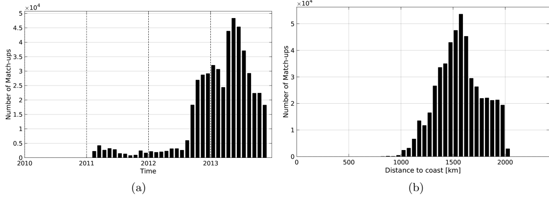
Figure 1: Number of match-ups between Surface drifters and SMOS-L3-CATDS-CPDC-V3-MONTHLY-25KM SSS as a function of time (a) and as function of the distance to coast (b) over the SPURS 1 Pi-MEP region and for the full satellite product period.
