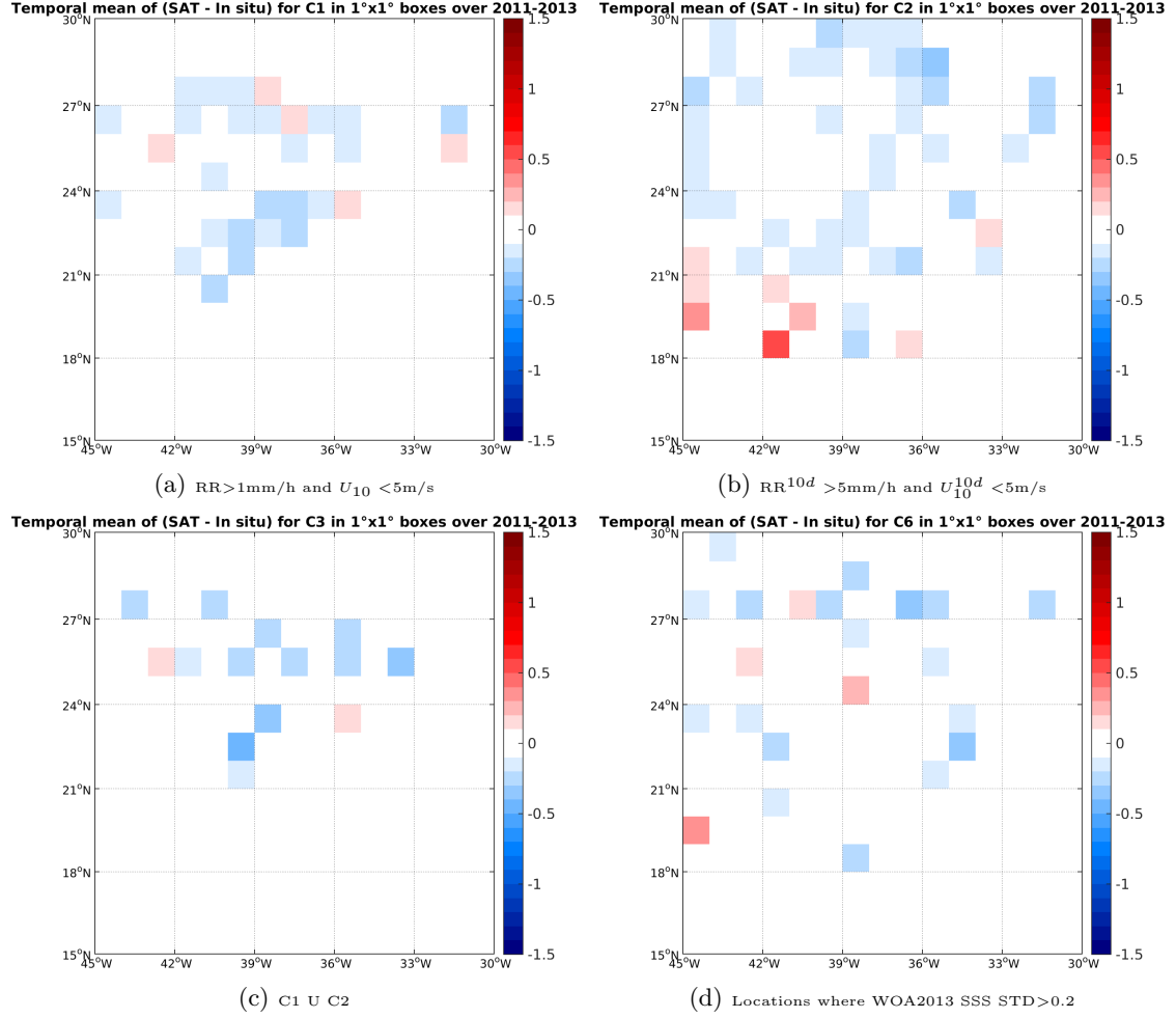
Figure 11: Temporal mean gridded over spatial boxes of size 1^\circ \times 1^\circ of \Delta SSS (SMOS-L3-CATDS-CPDC-V3-MONTHLY-25KM - Surface drifters) for 4 different subdatasets corresponding to: RR > 1 mm/h and U_{10} < 5 m/s (a), RR 10d > 5 mm/h and U_{10}^{10d} < 5 m/s (b), C1 U C2 (c), Locations where WOA2013 SSS STD > 0.2 (d).
