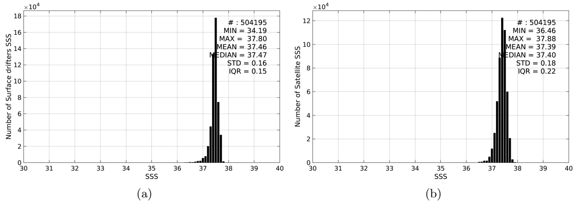
Figure 2: Histograms of SSS from Surface drifters (a) and SMOS-L3-CATDS-CPDC-V3-MONTHLY-25KM (b) considering all match-up pairs per bins of 0.1 over the SPURS 1 Pi-MEP region and for the full satellite product period.
