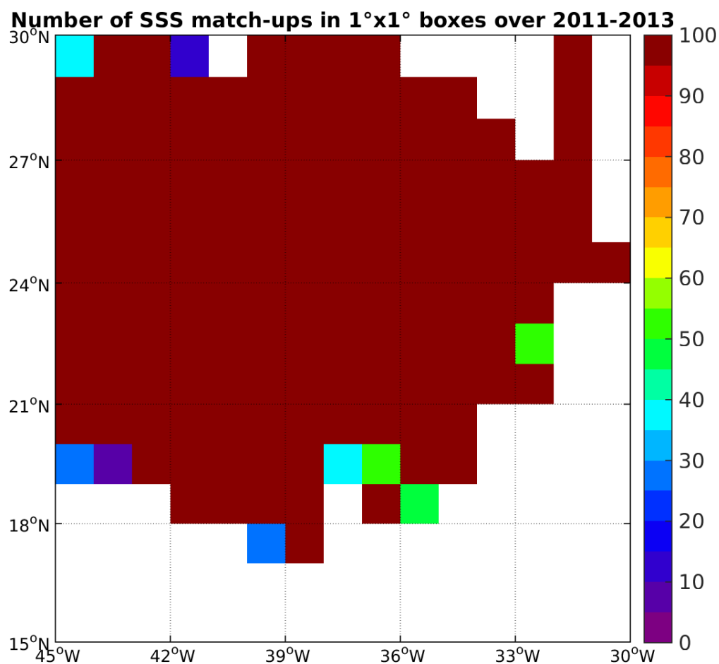
Figure 3: Number of SSS match-ups between Surface drifters SSS and the SMOS-L3-CATDS-CPDC-V3-MONTHLY-25KM SSS product for the SPURS 1 Pi-MEP region over 1°x1° boxes and for the full satellite product period.
