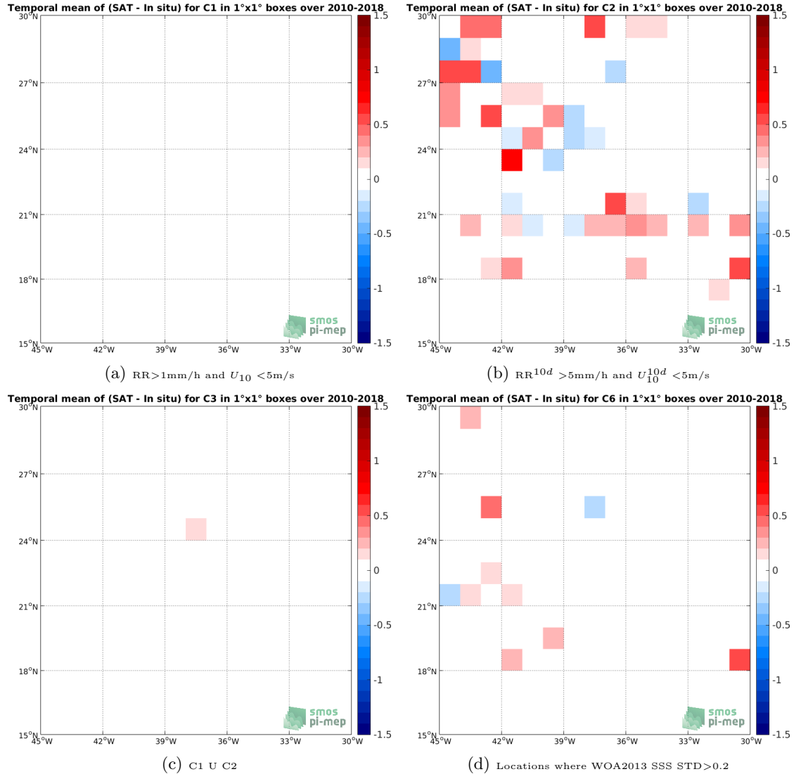
Figure 12: Temporal mean gridded over spatial boxes of size 1^\circ \times 1^\circ of \Delta SSS (SMOS-L3-CATDS-CPDC-V3-10DAYS-25KM - TSG-SAMOS) for 4 different subdatasets corresponding to: RR > 1\text{mm/h} and U_{10} < 5\text{m/s} (a), RR^{10d} > 5\text{mm/h} and U_{10}^{10d} < 5\text{m/s} (b), C1 U C2 (c), Locations where WOA2013 SSS STD > 0.2 (d).
