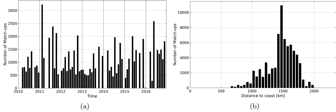
Figure 1: Number of match-ups between TSG-LEGOS-DM and SMOS-L3-CATDS-CPDC-V3-10DAYS-25KM SSS as a function of time (a) and as function of the distance to coast (b) over the SPURS 1 Pi-MEP region and for the full satellite product period.
