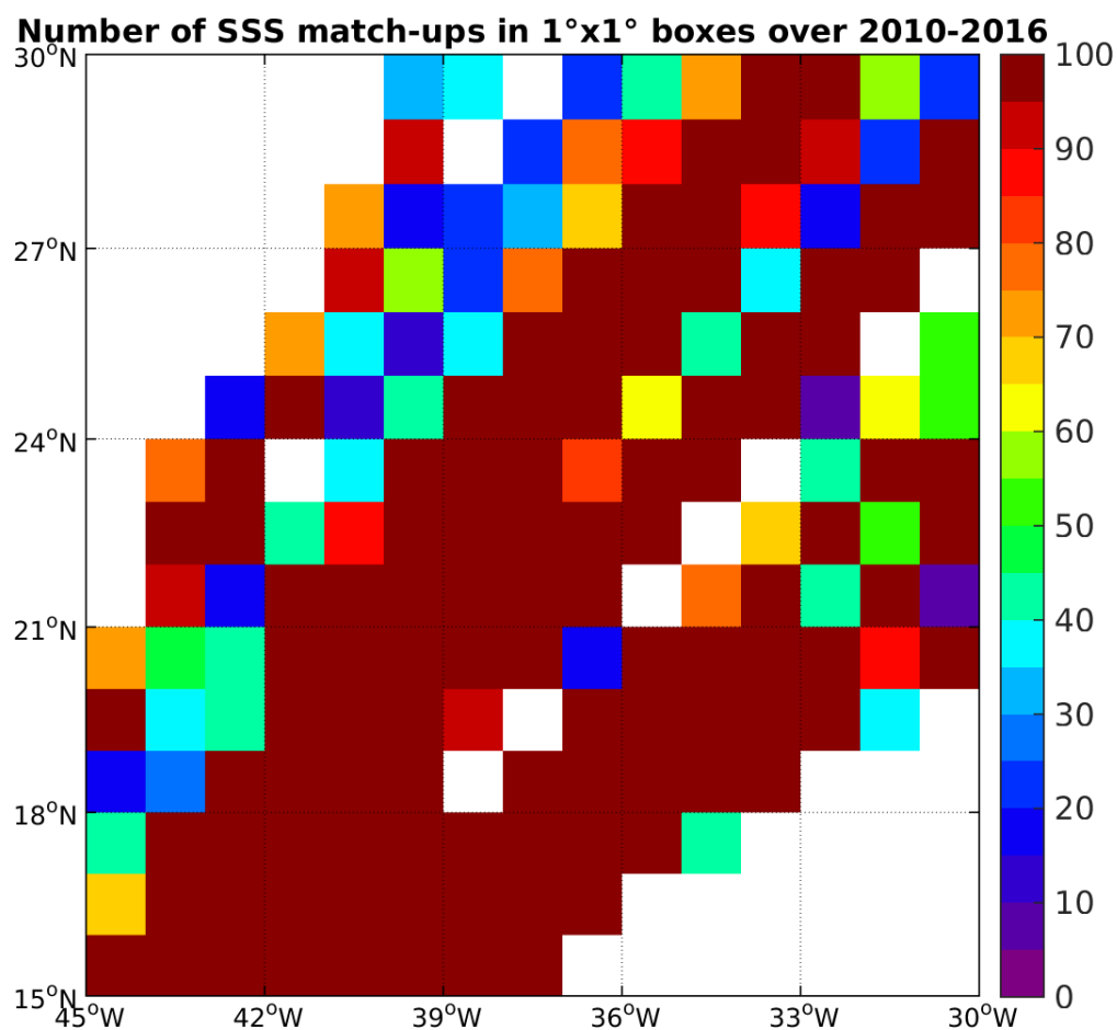
Figure 4: Number of SSS match-ups between TSG-LEGOS-DM SSS and the SMOS-L3-CATDS-CPDC-V3-10DAYS-25KM SSS product for the SPURS 1 Pi-MEP region over 1°x1° boxes and for the full satellite product period.
