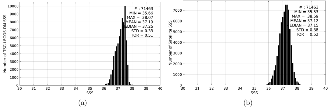
Figure 2: Histograms of SSS from TSG-LEGOS-DM (a) and SMOS-L3-CATDS-CPDC-V3-10DAYS-25KM (b) considering all match-up pairs per bins of 0.1 over the SPURS 1 Pi-MEP region and for the full satellite product period.
