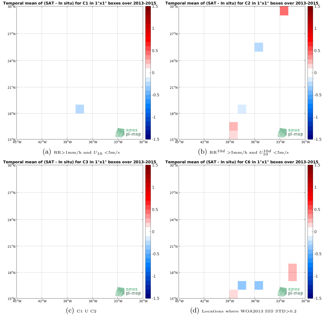
Figure 12: Temporal mean gridded over spatial boxes of size 1^\circ \times 1^\circ of \Delta\text{SSS} (SMOS-L3-CATDS-CPDC-V3-10DAYS-25KM - TSG-GOSUD-Sailing-ship) for 4 different subdatasets corresponding to: RR > 1\text{mm/h} and U_{10} < 5\text{m/s} (a), RR^{10d} > 5\text{mm/h} and U_{10}^{10d} < 5\text{m/s} (b), C1 U C2 (c), Locations where WOA2013 SSS STD > 0.2 (d).
