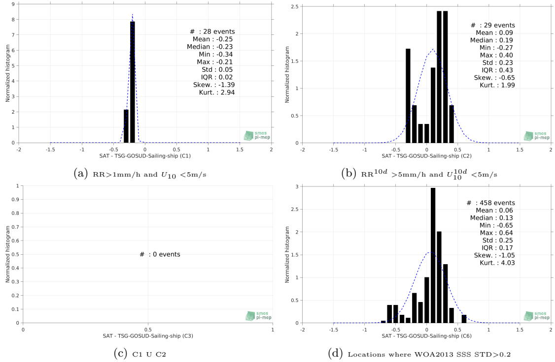
Figure 13: Normalized histogram of \Delta\text{SSS} (SMOS-L3-CATDS-CPDC-V3-10DAYS-25KM - TSG-GOSUD-Sailing-ship) for 6 different subdatasets corresponding to: RR > 1\text{mm/h} and U_{10} < 5\text{m/s} (a), RR^{10d} > 5\text{mm/h} and U_{10}^{10d} < 5\text{m/s} (b), C1 U C2 (c), Locations where WOA2013 SSS STD > 0.2 (d).
